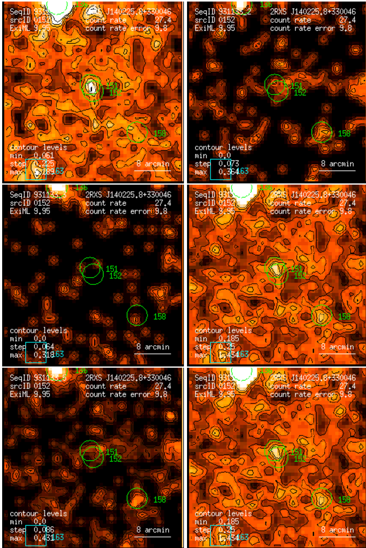
Figure 152: RASS 931133: detection 0152: band rate images, Gaussian filter: (1) PSPC channels 11 – 41, (2) 52 – 90, (3) 91 – 201, (4) 11 – 235, (5) 52 – 201, (6) 11 – 201. Broad band rates in counts/ks. Band rate contour levels in counts/ks/arcmin 2 .
