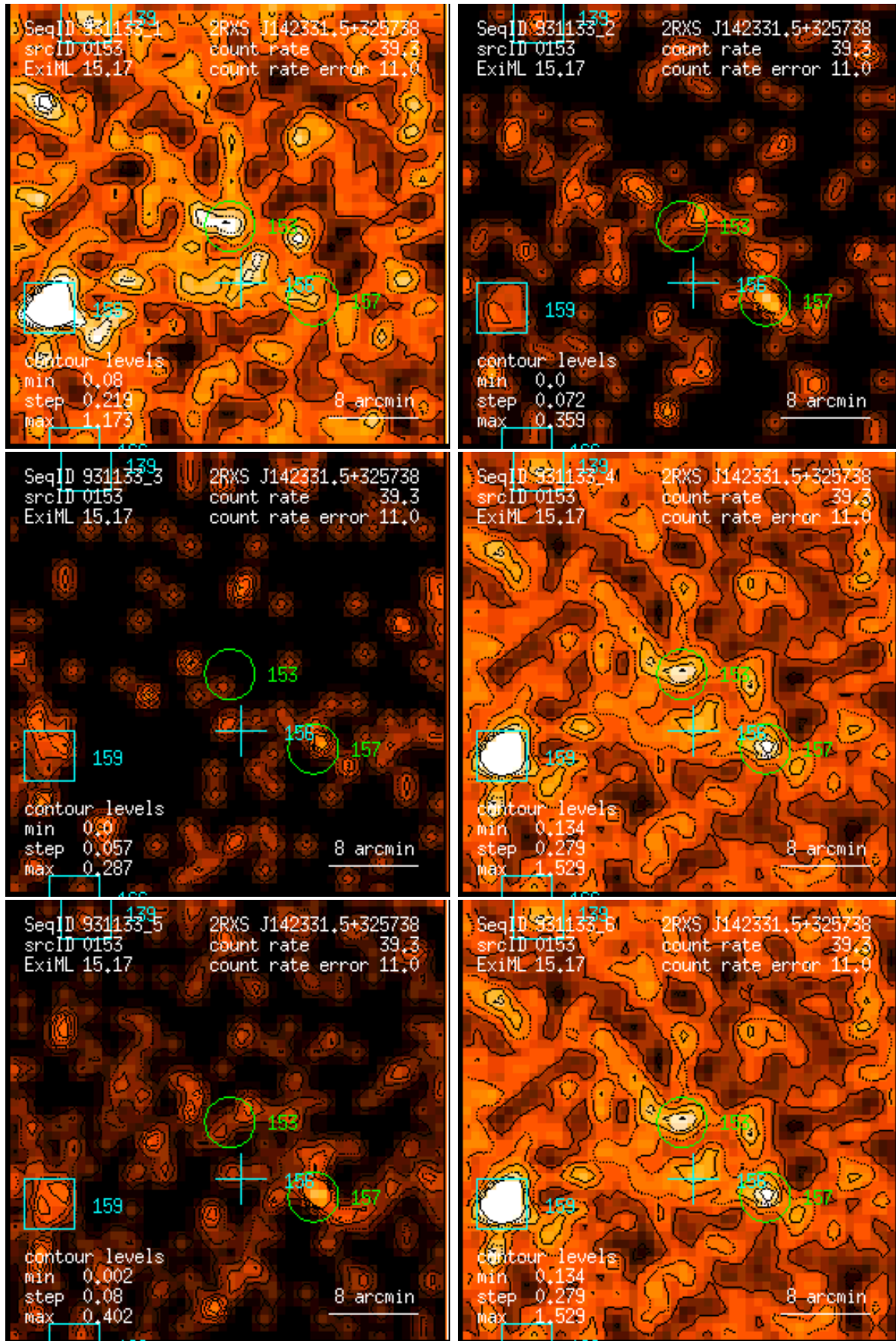
Figure 153: RASS 931133: detection 0153: band rate images, Gaussian filter: (1) PSPC channels 11 – 41, (2) 52 – 90, (3) 91 – 201, (4) 11 – 235, (5) 52 – 201, (6) 11 – 201. Broad band rates in counts/ks. Band rate contour levels in counts/ks/arcmin 2 .
