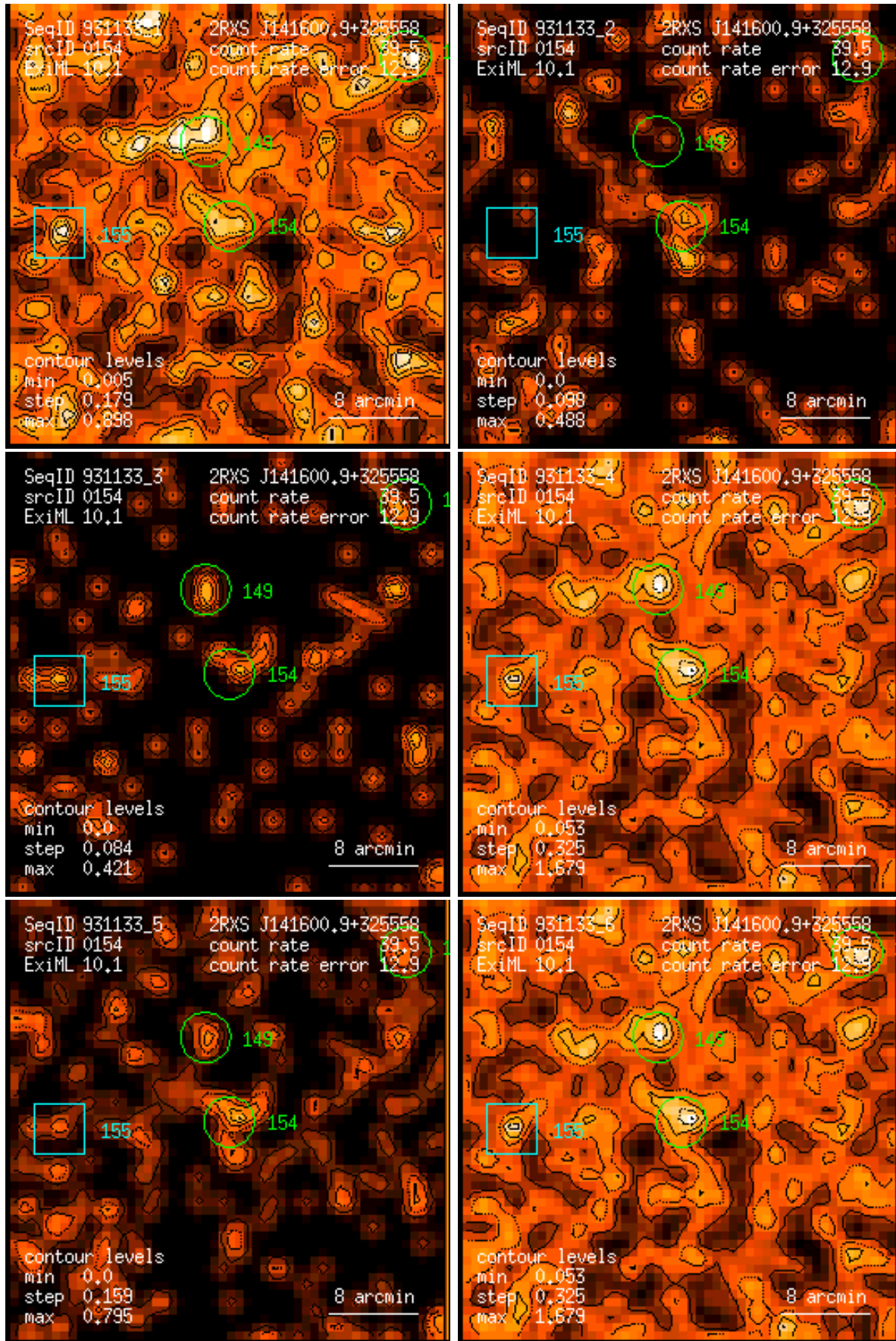
Figure 154: RASS 931133: detection 0154: band rate images, Gaussian filter: (1) PSPC channels 11 – 41, (2) 52 – 90, (3) 91 – 201, (4) 11 – 235, (5) 52 – 201, (6) 11 – 201. Broad band rates in counts/ks. Band rate contour levels in counts/ks/arcmin 2 .
