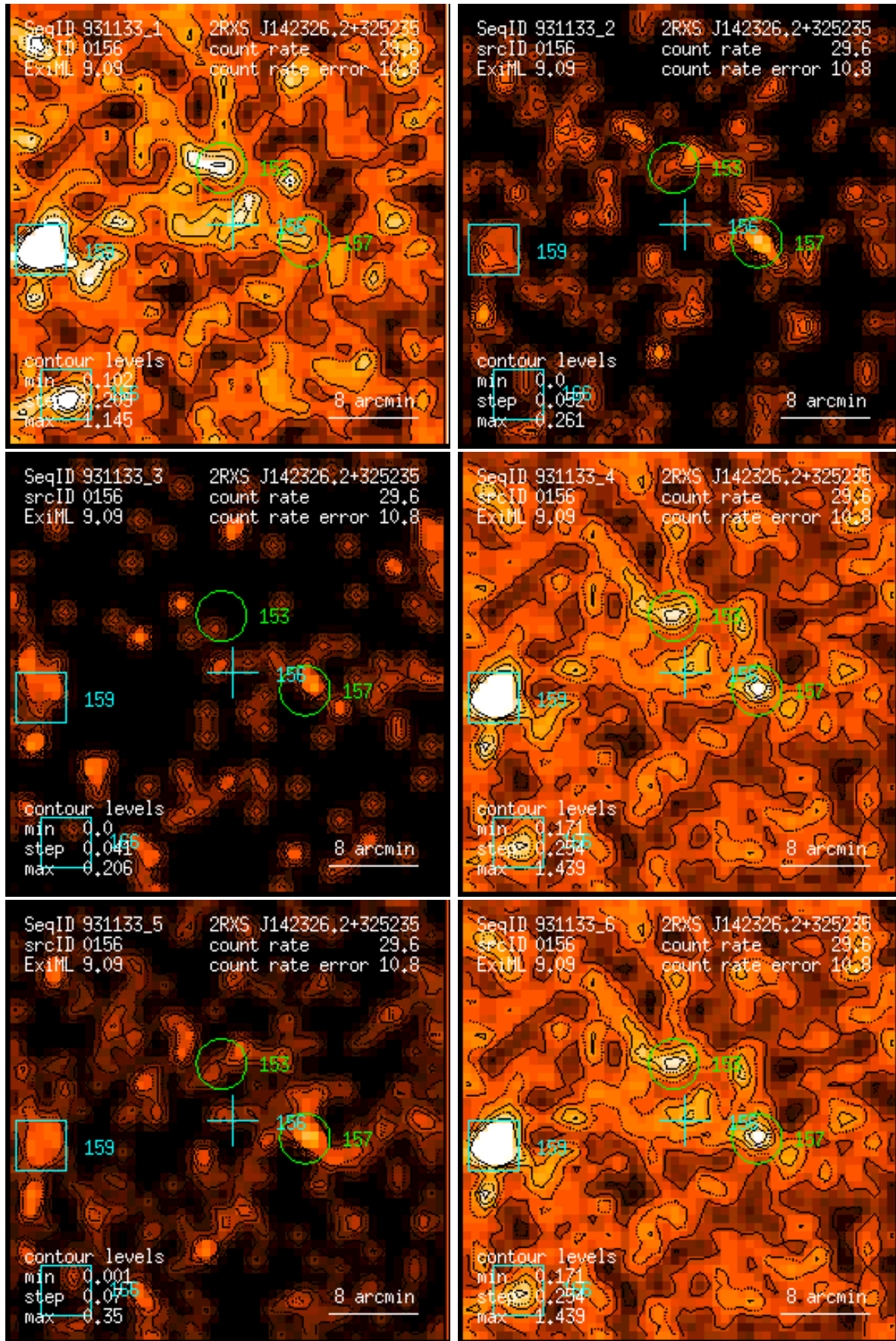
Figure 156: RASS 931133: detection 0156: band rate images, Gaussian filter: (1) PSPC channels 11 – 41, (2) 52 – 90, (3) 91 – 201, (4) 11 – 235, (5) 52 – 201, (6) 11 – 201. Broad band rates in counts/ks. Band rate contour levels in counts/ks/arcmin 2 .
