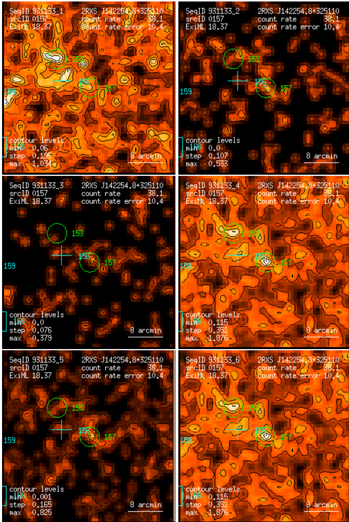
Figure 157: RASS 931133: detection 0157: band rate images, Gaussian filter: (1) PSPC channels 11 – 41, (2) 52 – 90, (3) 91 – 201, (4) 11 – 235, (5) 52 – 201, (6) 11 – 201. Broad band rates in counts/ks. Band rate contour levels in counts/ks/arcmin 2 .
