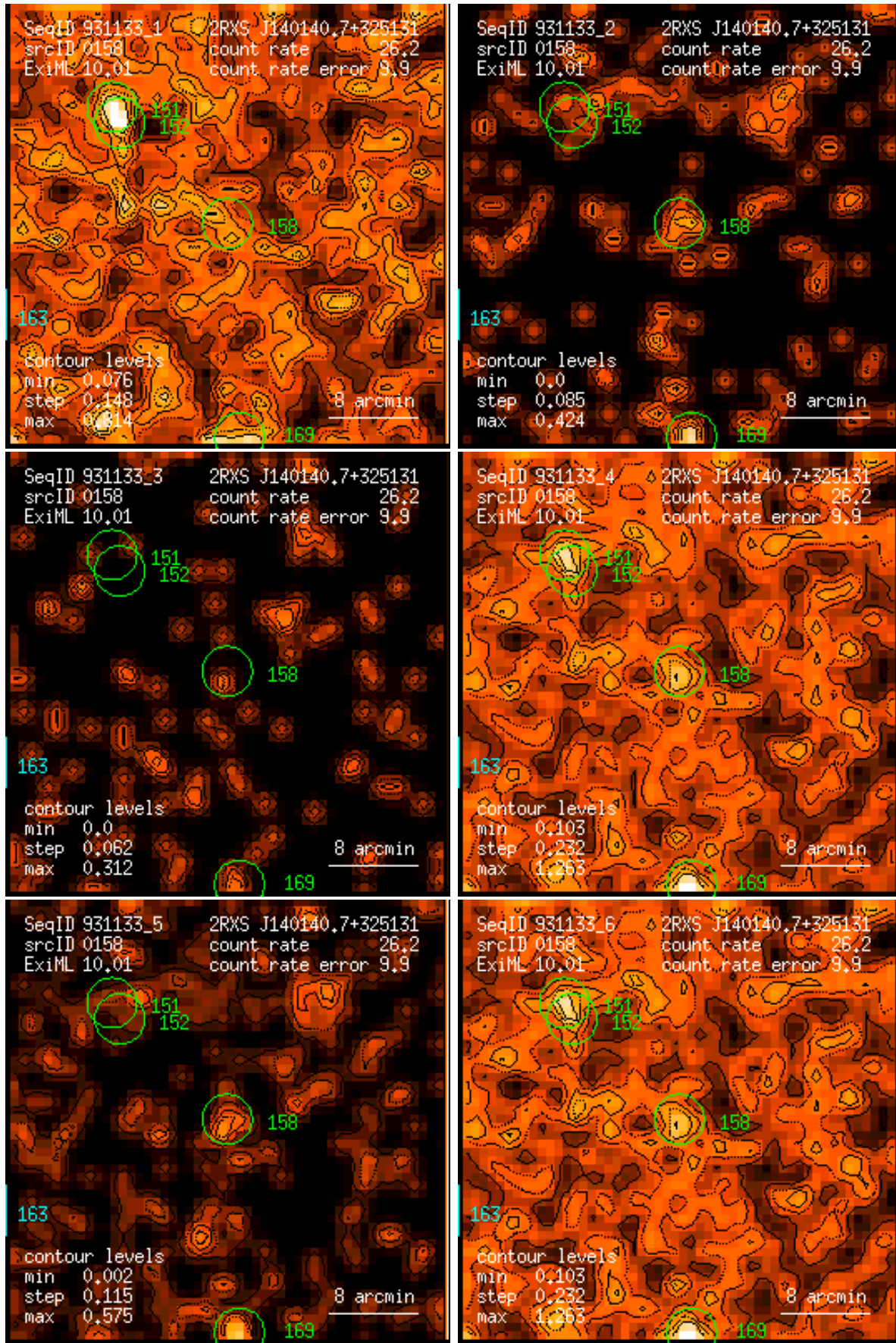
Figure 158: RASS 931133: detection 0158: band rate images, Gaussian filter: (1) PSPC channels 11 – 41, (2) 52 – 90, (3) 91 – 201, (4) 11 – 235, (5) 52 – 201, (6) 11 – 201. Broad band rates in counts/ks. Band rate contour levels in counts/ks/arcmin 2 .
