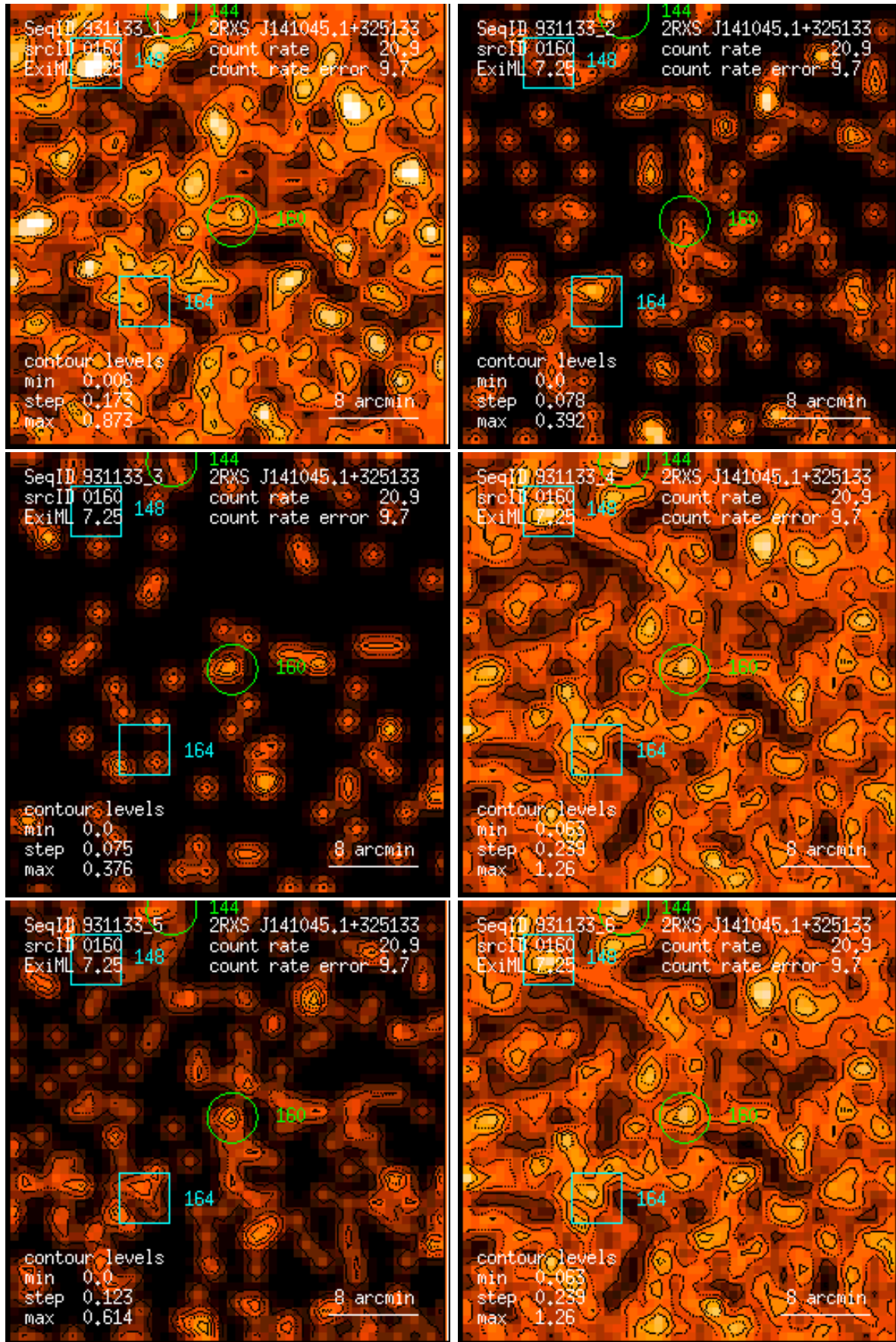
Figure 160: RASS 931133: detection 0160: band rate images, Gaussian filter: (1) PSPC channels 11 – 41, (2) 52 – 90, (3) 91 – 201, (4) 11 – 235, (5) 52 – 201, (6) 11 – 201. Broad band rates in counts/ks. Band rate contour levels in counts/ks/arcmin 2 .
