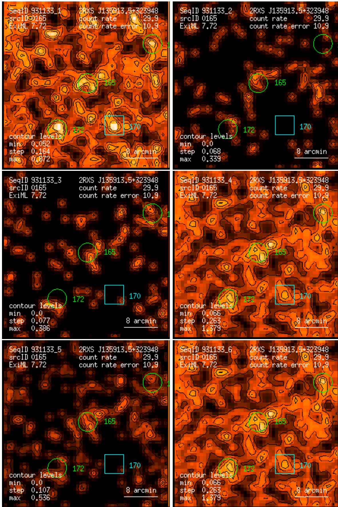
Figure 165: RASS 931133: detection 0165: band rate images, Gaussian filter: (1) PSPC channels 11 – 41, (2) 52 – 90, (3) 91 – 201, (4) 11 – 235, (5) 52 – 201, (6) 11 – 201. Broad band rates in counts/ks. Band rate contour levels in counts/ks/arcmin 2 .
