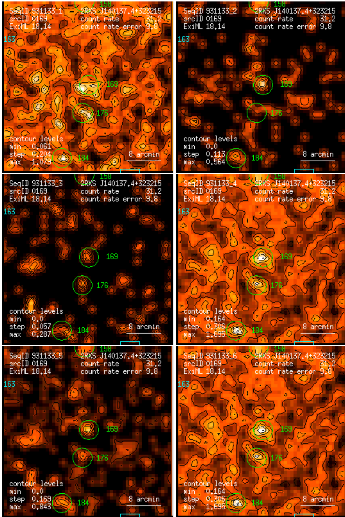
Figure 169: RASS 931133: detection 0169: band rate images, Gaussian filter: (1) PSPC channels 11 – 41, (2) 52 – 90, (3) 91 – 201, (4) 11 – 235, (5) 52 – 201, (6) 11 – 201. Broad band rates in counts/ks. Band rate contour levels in counts/ks/arcmin 2 .
