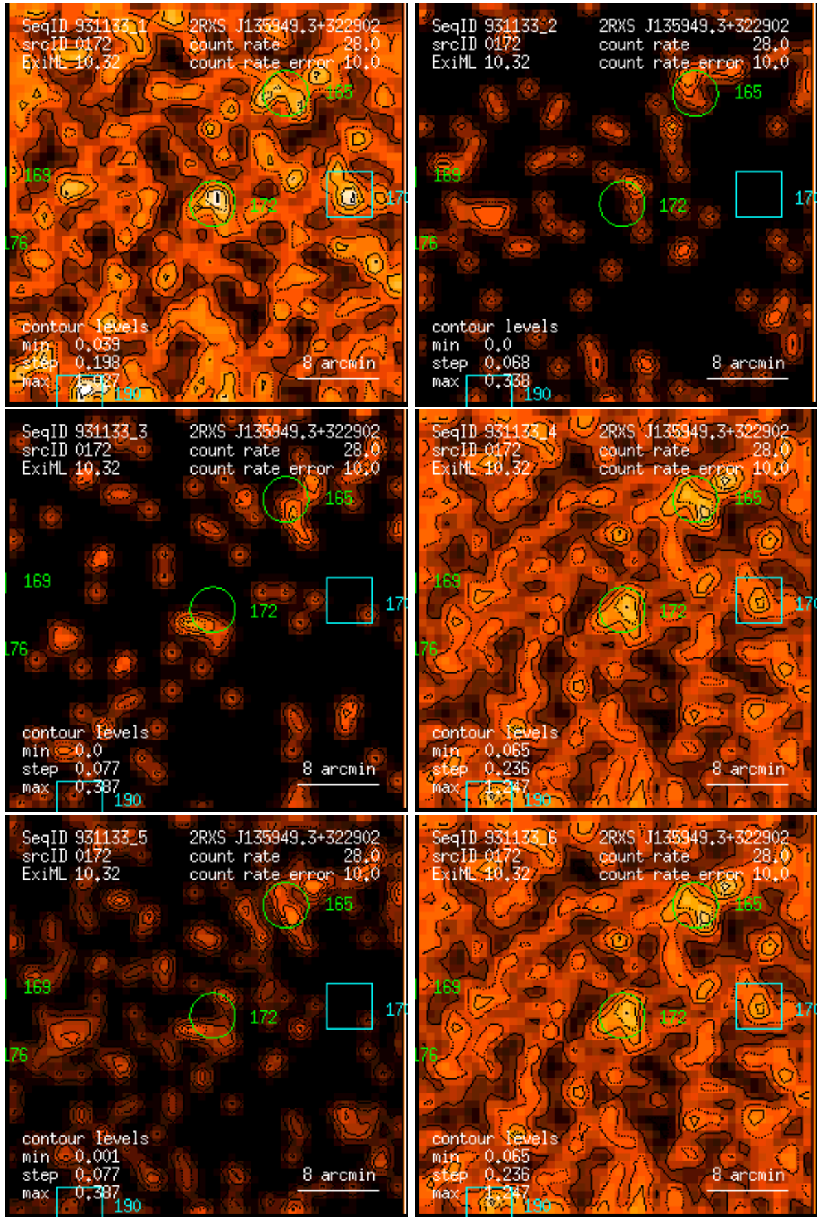
Figure 172: RASS 931133: detection 0172: band rate images, Gaussian filter: (1) PSPC channels 11 – 41, (2) 52 – 90, (3) 91 – 201, (4) 11 – 235, (5) 52 – 201, (6) 11 – 201. Broad band rates in counts/ks. Band rate contour levels in counts/ks/arcmin 2 .
