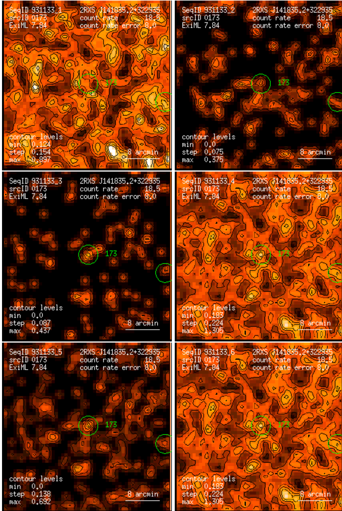
Figure 173: RASS 931133: detection 0173: band rate images, Gaussian filter: (1) PSPC channels 11 – 41, (2) 52 – 90, (3) 91 – 201, (4) 11 – 235, (5) 52 – 201, (6) 11 – 201. Broad band rates in counts/ks. Band rate contour levels in counts/ks/arcmin 2 .
