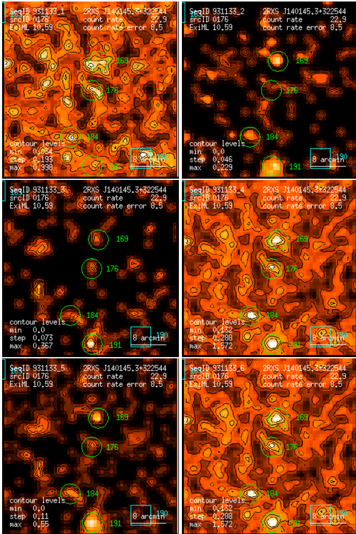
Figure 176: RASS 931133: detection 0176: band rate images, Gaussian filter: (1) PSPC channels 11 – 41, (2) 52 – 90, (3) 91 – 201, (4) 11 – 235, (5) 52 – 201, (6) 11 – 201. Broad band rates in counts/ks. Band rate contour levels in counts/ks/arcmin 2 .
