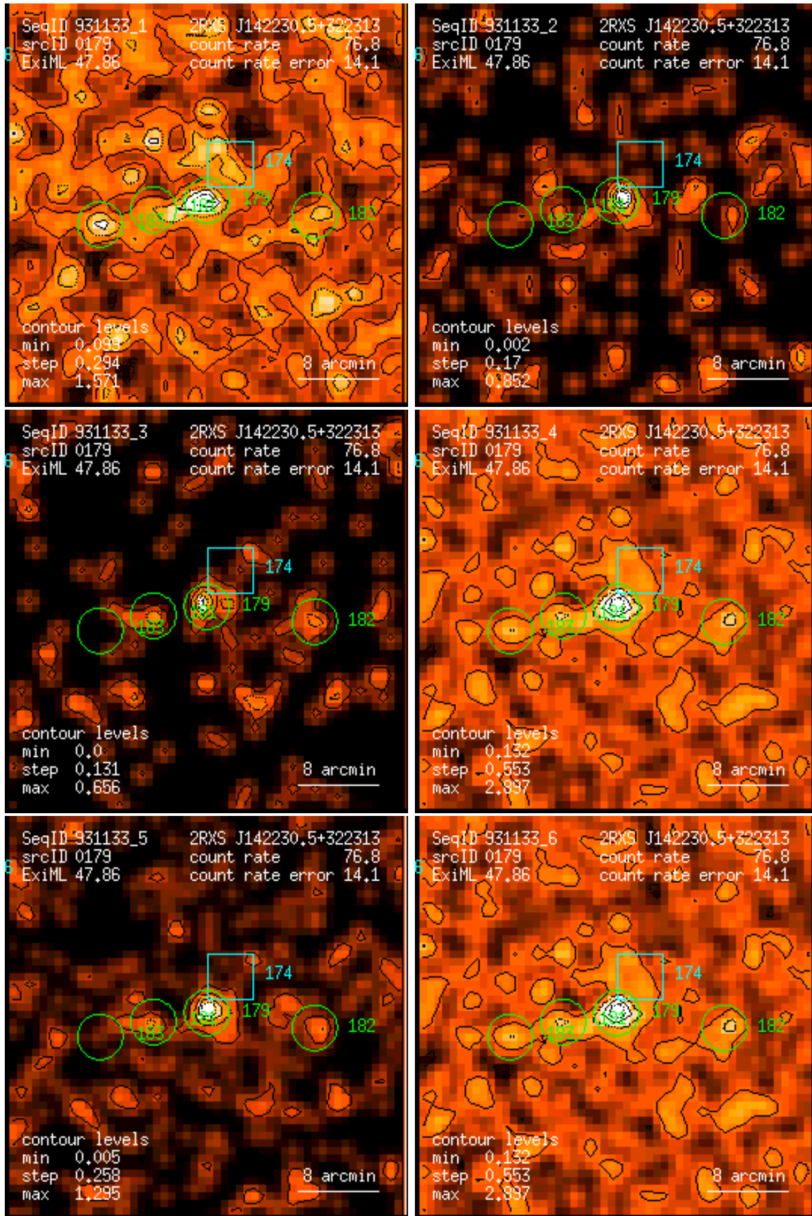
Figure 179: RASS 931133: detection 0179: band rate images, Gaussian filter: (1) PSPC channels 11 – 41, (2) 52 – 90, (3) 91 – 201, (4) 11 – 235, (5) 52 – 201, (6) 11 – 201. Broad band rates in counts/ks. Band rate contour levels in counts/ks/arcmin 2 .
