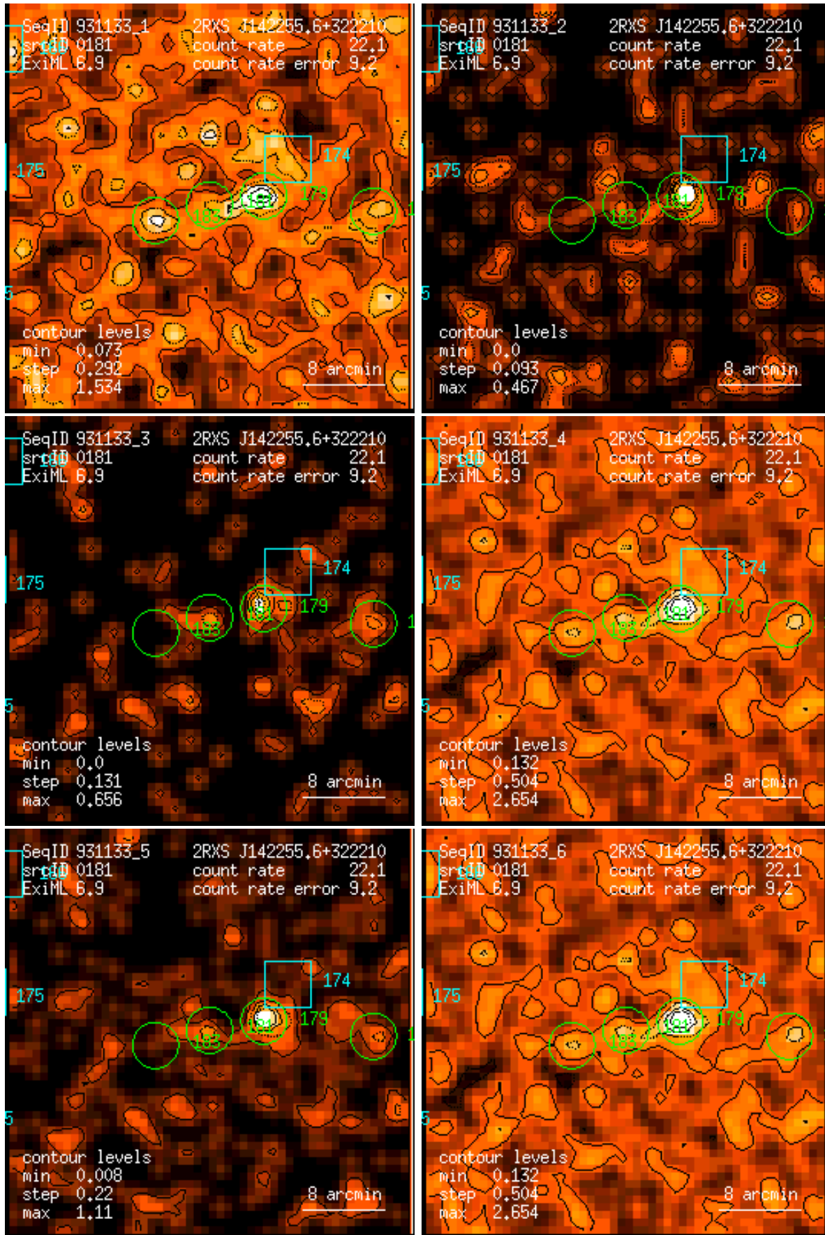
Figure 181: RASS 931133: detection 0181: band rate images, Gaussian filter: (1) PSPC channels 11 – 41, (2) 52 – 90, (3) 91 – 201, (4) 11 – 235, (5) 52 – 201, (6) 11 – 201. Broad band rates in counts/ks. Band rate contour levels in counts/ks/arcmin 2 .
