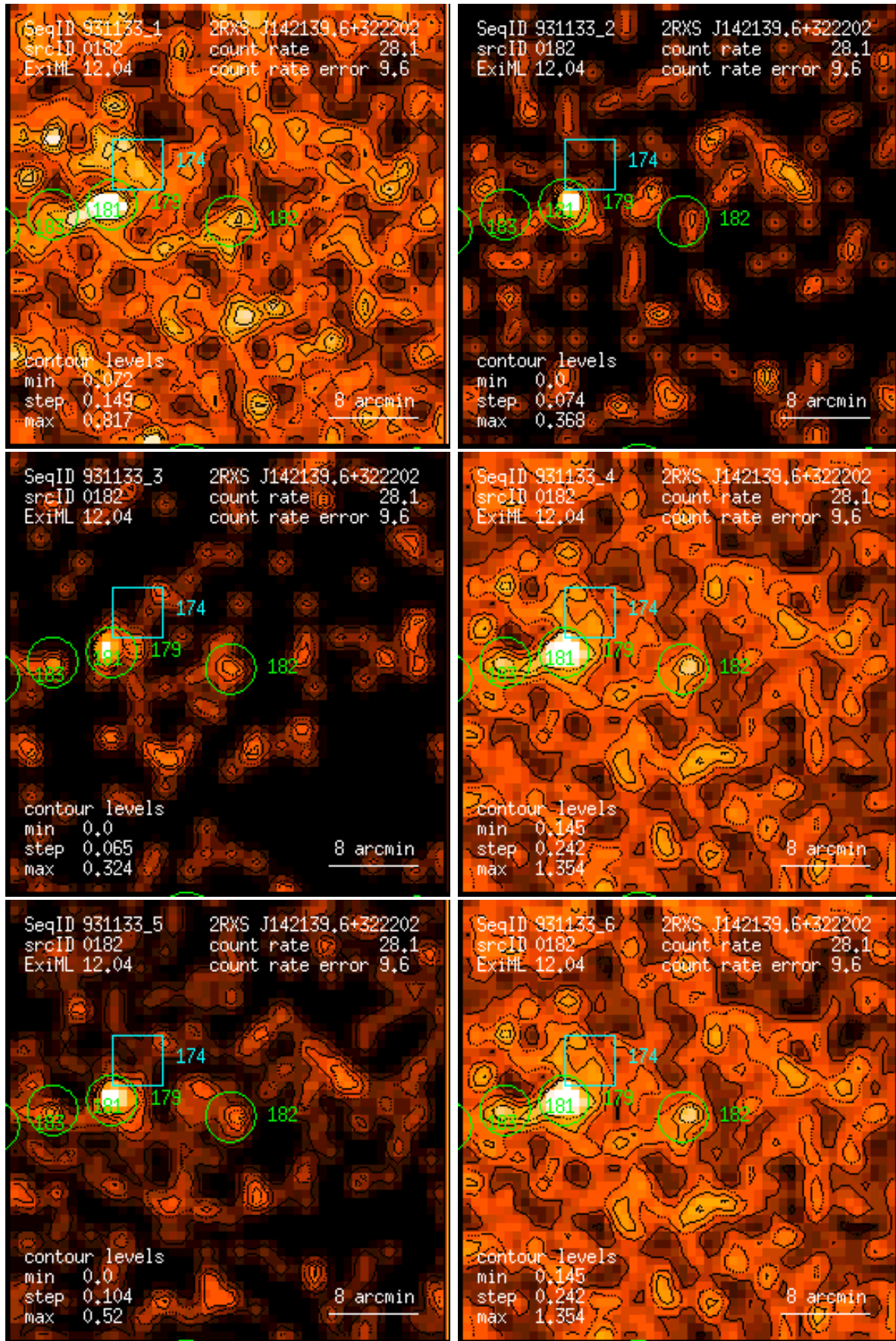
Figure 182: RASS 931133: detection 0182: band rate images, Gaussian filter: (1) PSPC channels 11 – 41, (2) 52 – 90, (3) 91 – 201, (4) 11 – 235, (5) 52 – 201, (6) 11 – 201. Broad band rates in counts/ks. Band rate contour levels in counts/ks/arcmin 2 .
