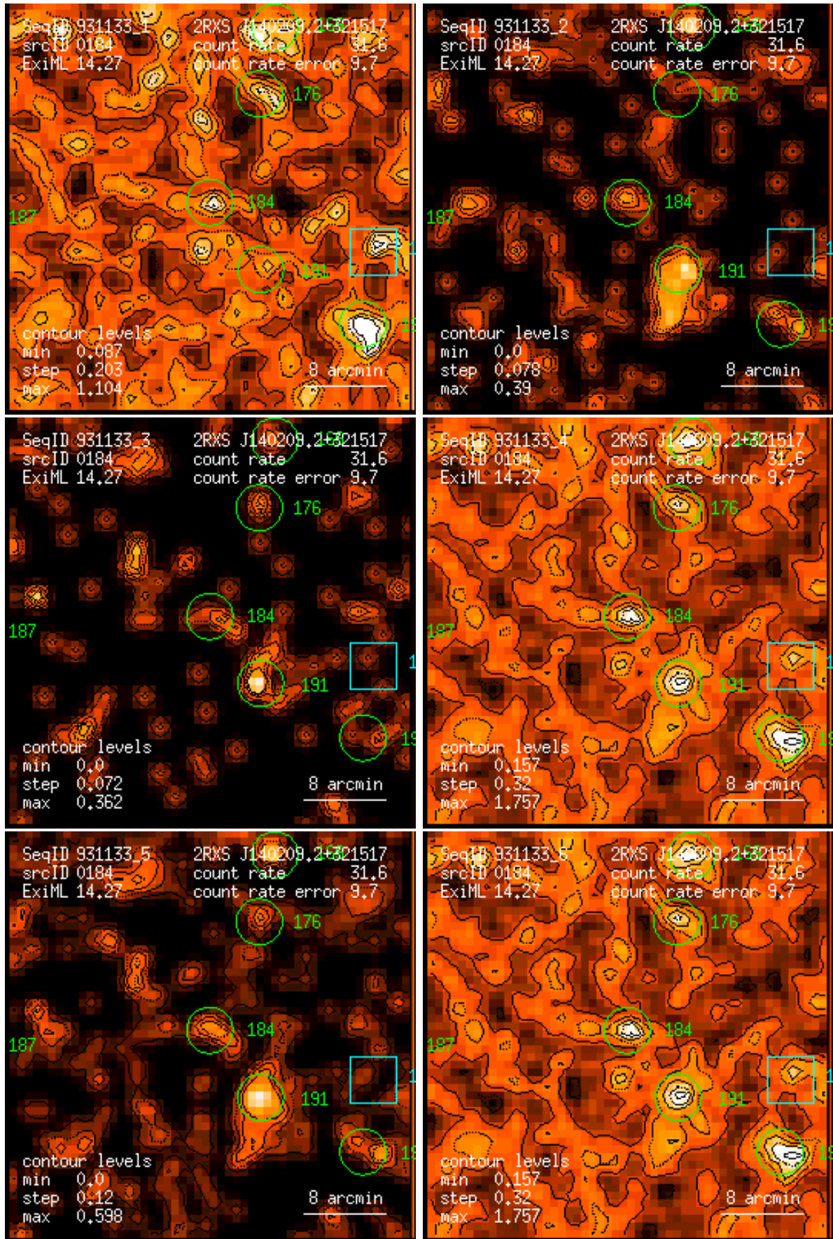
Figure 184: RASS 931133: detection 0184: band rate images, Gaussian filter: (1) PSPC channels 11 – 41, (2) 52 – 90, (3) 91 – 201, (4) 11 – 235, (5) 52 – 201, (6) 11 – 201. Broad band rates in counts/ks. Band rate contour levels in counts/ks/arcmin 2 .
