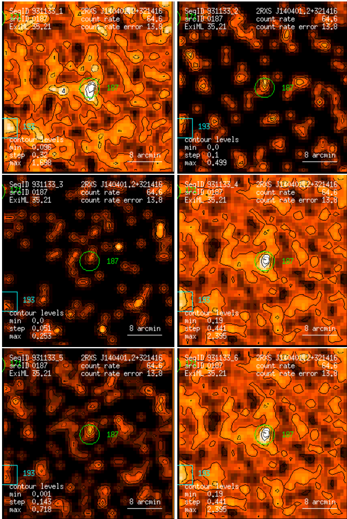
Figure 187: RASS 931133: detection 0187: band rate images, Gaussian filter: (1) PSPC channels 11 – 41, (2) 52 – 90, (3) 91 – 201, (4) 11 – 235, (5) 52 – 201, (6) 11 – 201. Broad band rates in counts/ks. Band rate contour levels in counts/ks/arcmin 2 .
