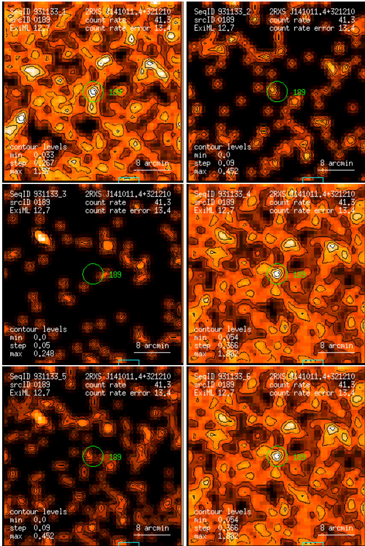
Figure 189: RASS 931133: detection 0189: band rate images, Gaussian filter: (1) PSPC channels 11 – 41, (2) 52 – 90, (3) 91 – 201, (4) 11 – 235, (5) 52 – 201, (6) 11 – 201. Broad band rates in counts/ks. Band rate contour levels in counts/ks/arcmin 2 .
