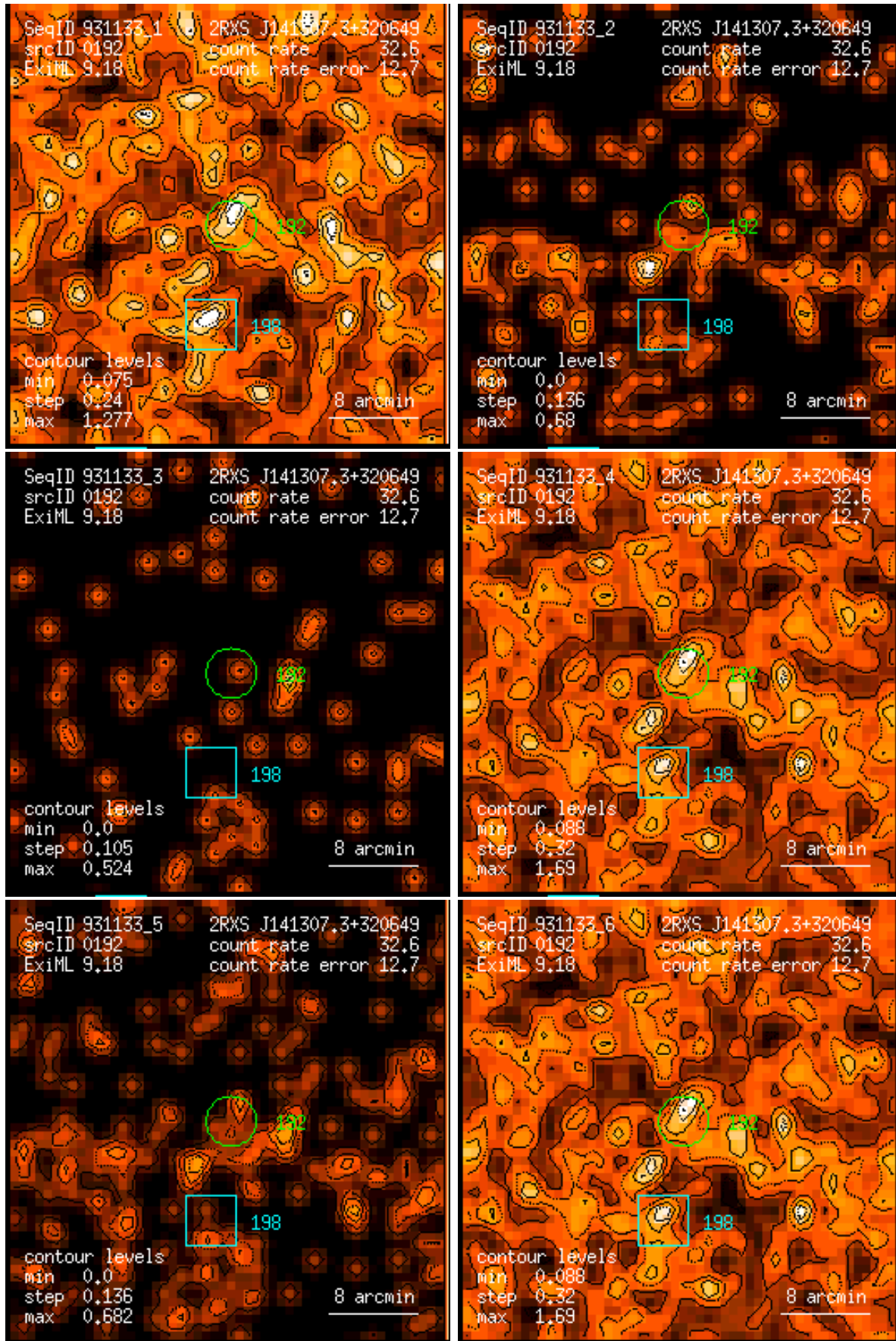
Figure 192: RASS 931133: detection 0192: band rate images, Gaussian filter: (1) PSPC channels 11 – 41, (2) 52 – 90, (3) 91 – 201, (4) 11 – 235, (5) 52 – 201, (6) 11 – 201. Broad band rates in counts/ks. Band rate contour levels in counts/ks/arcmin 2 .
