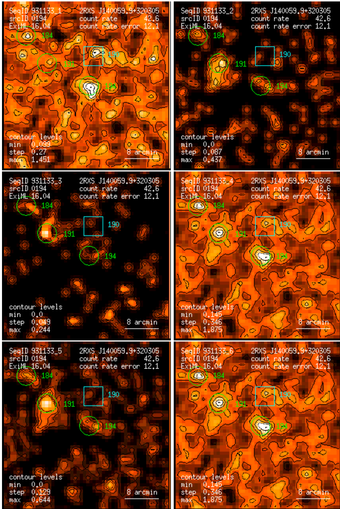
Figure 194: RASS 931133: detection 0194: band rate images, Gaussian filter: (1) PSPC channels 11 – 41, (2) 52 – 90, (3) 91 – 201, (4) 11 – 235, (5) 52 – 201, (6) 11 – 201. Broad band rates in counts/ks. Band rate contour levels in counts/ks/arcmin 2 .
