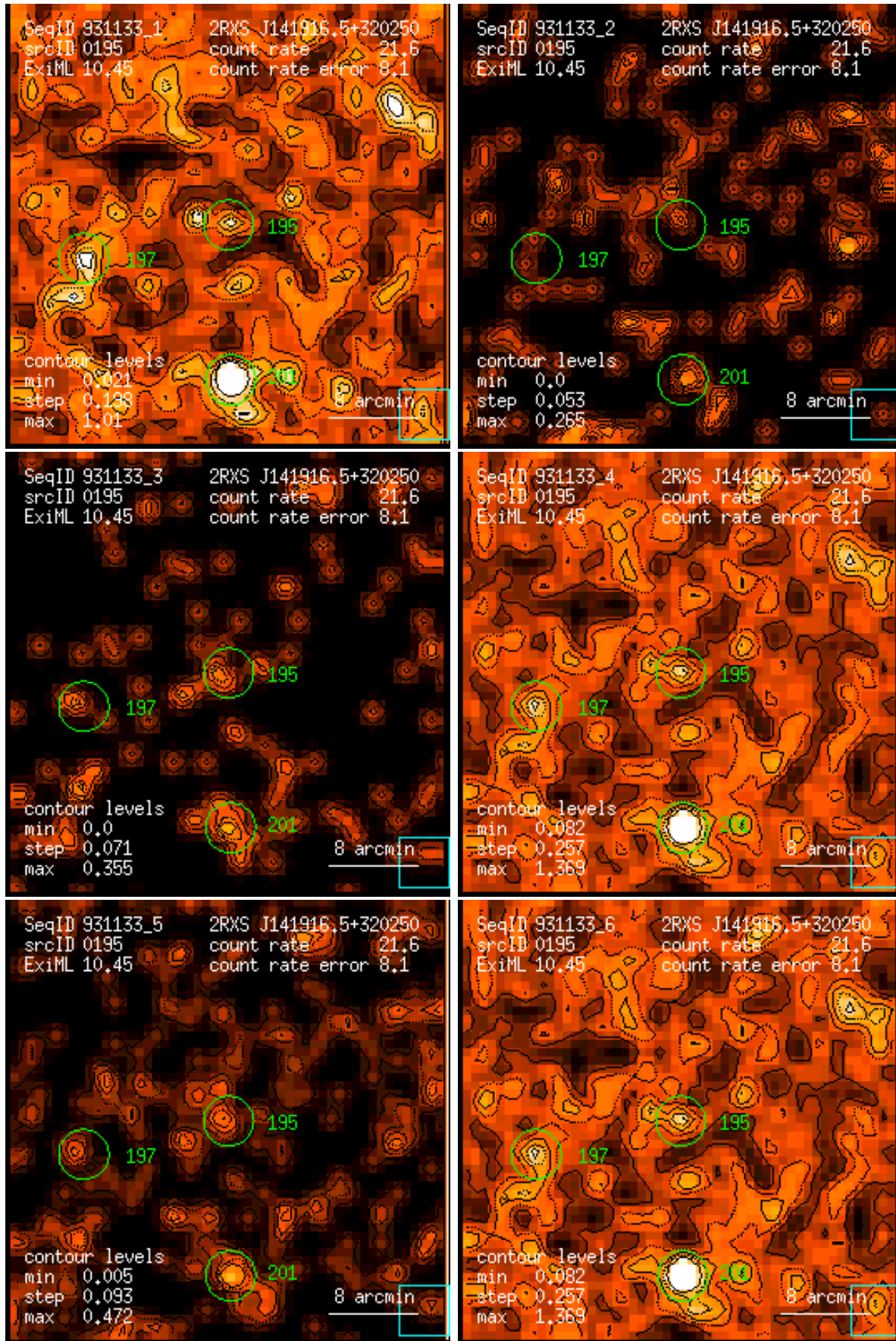
Figure 195: RASS 931133: detection 0195: band rate images, Gaussian filter: (1) PSPC channels 11 – 41, (2) 52 – 90, (3) 91 – 201, (4) 11 – 235, (5) 52 – 201, (6) 11 – 201. Broad band rates in counts/ks. Band rate contour levels in counts/ks/arcmin 2 .
