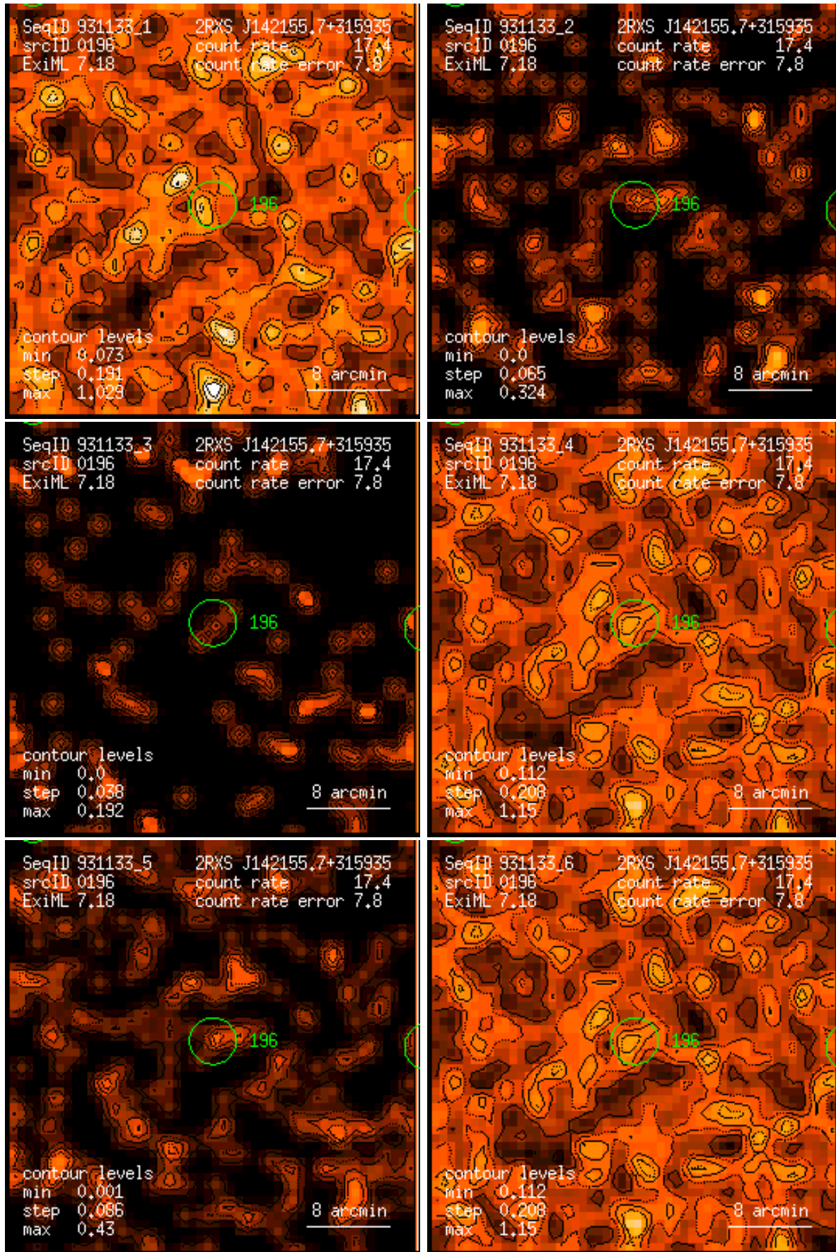
Figure 196: RASS 931133: detection 0196: band rate images, Gaussian filter: (1) PSPC channels 11 – 41, (2) 52 – 90, (3) 91 – 201, (4) 11 – 235, (5) 52 – 201, (6) 11 – 201. Broad band rates in counts/ks. Band rate contour levels in counts/ks/arcmin 2 .
