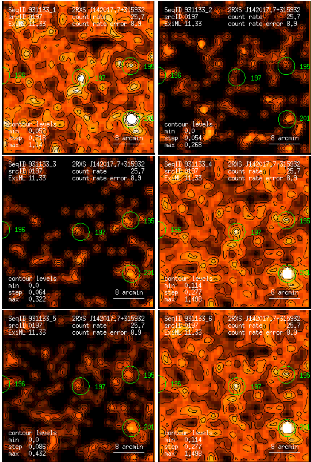
Figure 197: RASS 931133: detection 0197: band rate images, Gaussian filter: (1) PSPC channels 11 – 41, (2) 52 – 90, (3) 91 – 201, (4) 11 – 235, (5) 52 – 201, (6) 11 – 201. Broad band rates in counts/ks. Band rate contour levels in counts/ks/arcmin 2 .
