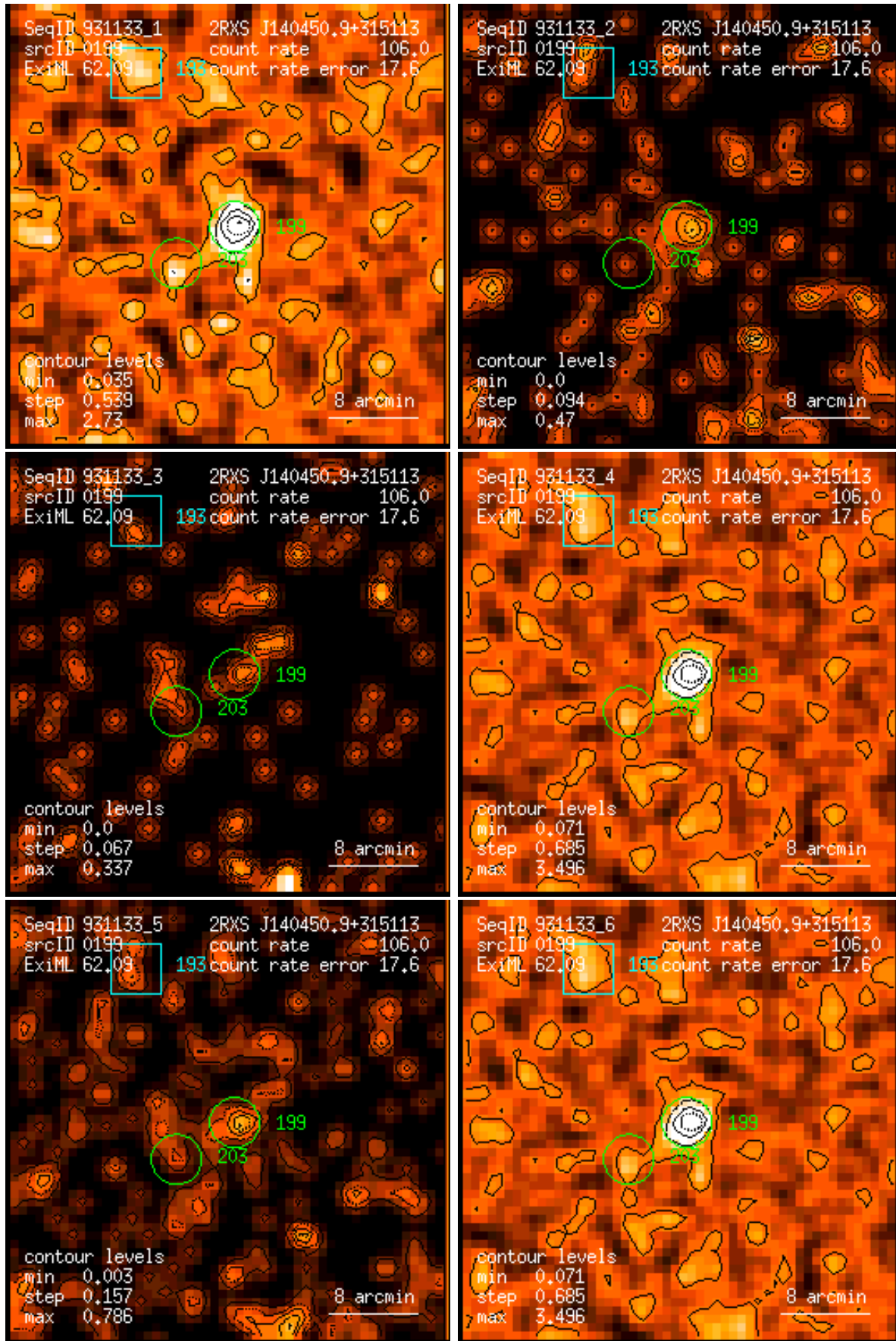
Figure 199: RASS 931133: detection 0199: band rate images, Gaussian filter: (1) PSPC channels 11 – 41, (2) 52 – 90, (3) 91 – 201, (4) 11 – 235, (5) 52 – 201, (6) 11 – 201. Broad band rates in counts/ks. Band rate contour levels in counts/ks/arcmin 2 .
