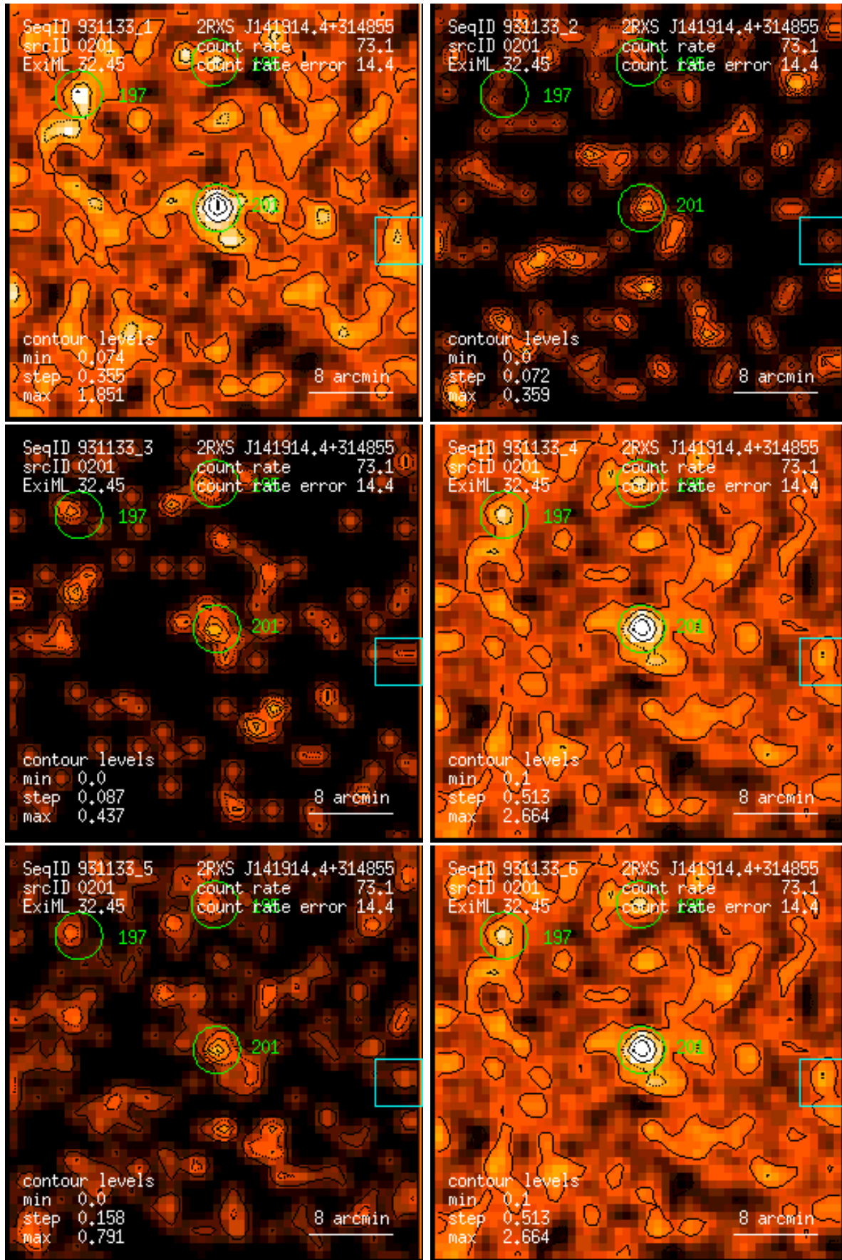
Figure 201: RASS 931133: detection 0201: band rate images, Gaussian filter: (1) PSPC channels 11 – 41, (2) 52 – 90, (3) 91 – 201, (4) 11 – 235, (5) 52 – 201, (6) 11 – 201. Broad band rates in counts/ks. Band rate contour levels in counts/ks/arcmin 2 .
