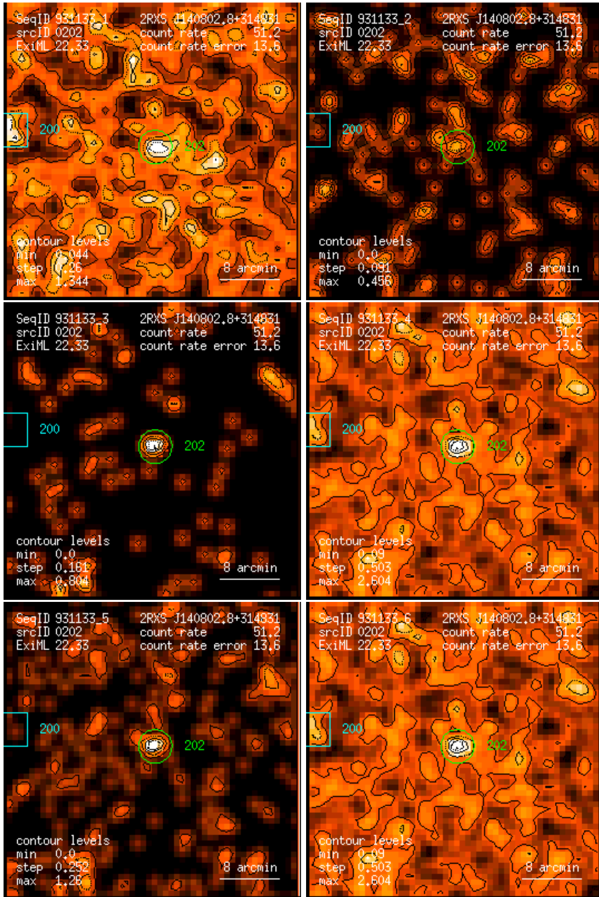
Figure 202: RASS 931133: detection 0202: band rate images, Gaussian filter: (1) PSPC channels 11 – 41, (2) 52 – 90, (3) 91 – 201, (4) 11 – 235, (5) 52 – 201, (6) 11 – 201. Broad band rates in counts/ks. Band rate contour levels in counts/ks/arcmin 2 .
