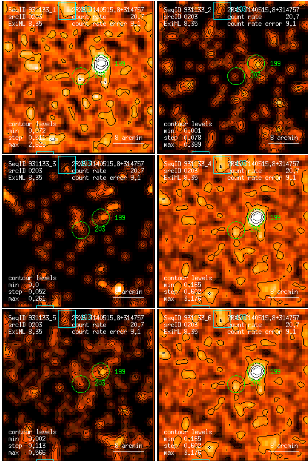
Figure 203: RASS 931133: detection 0203: band rate images, Gaussian filter: (1) PSPC channels 11 – 41, (2) 52 – 90, (3) 91 – 201, (4) 11 – 235, (5) 52 – 201, (6) 11 – 201. Broad band rates in counts/ks. Band rate contour levels in counts/ks/arcmin 2 .
