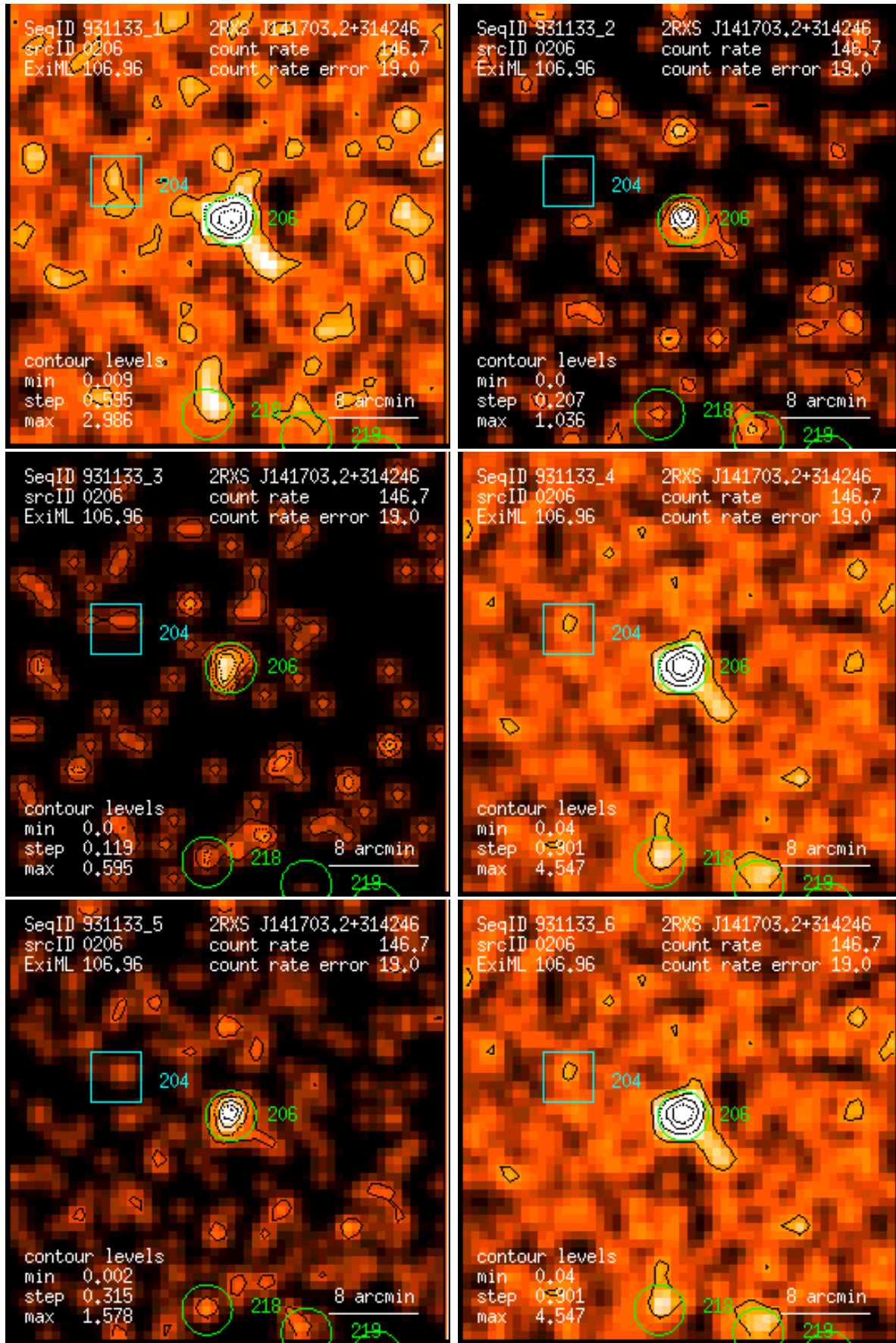
Figure 206: RASS 931133: detection 0206: band rate images, Gaussian filter: (1) PSPC channels 11 – 41, (2) 52 – 90, (3) 91 – 201, (4) 11 – 235, (5) 52 – 201, (6) 11 – 201. Broad band rates in counts/ks. Band rate contour levels in counts/ks/arcmin 2 .
