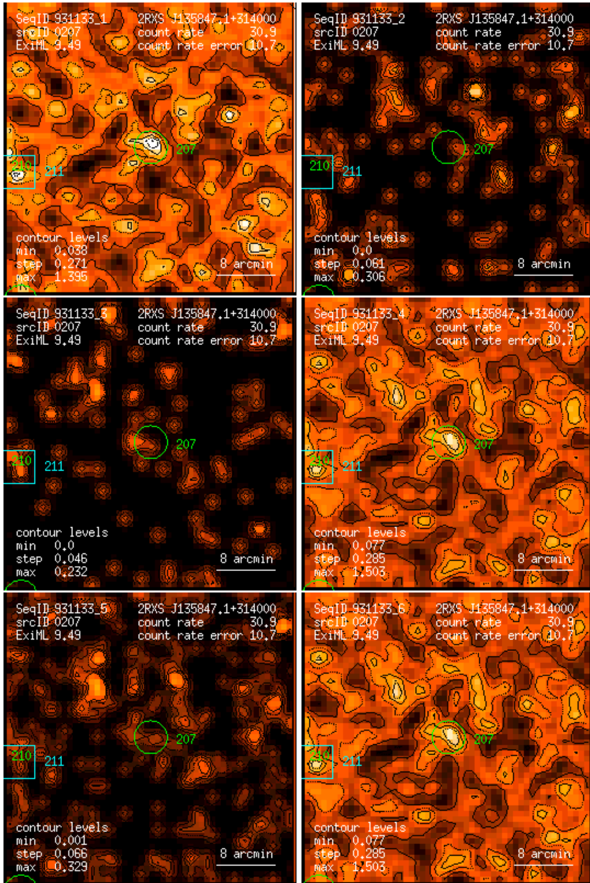
Figure 207: RASS 931133: detection 0207: band rate images, Gaussian filter: (1) PSPC channels 11 – 41, (2) 52 – 90, (3) 91 – 201, (4) 11 – 235, (5) 52 – 201, (6) 11 – 201. Broad band rates in counts/ks. Band rate contour levels in counts/ks/arcmin 2 .
