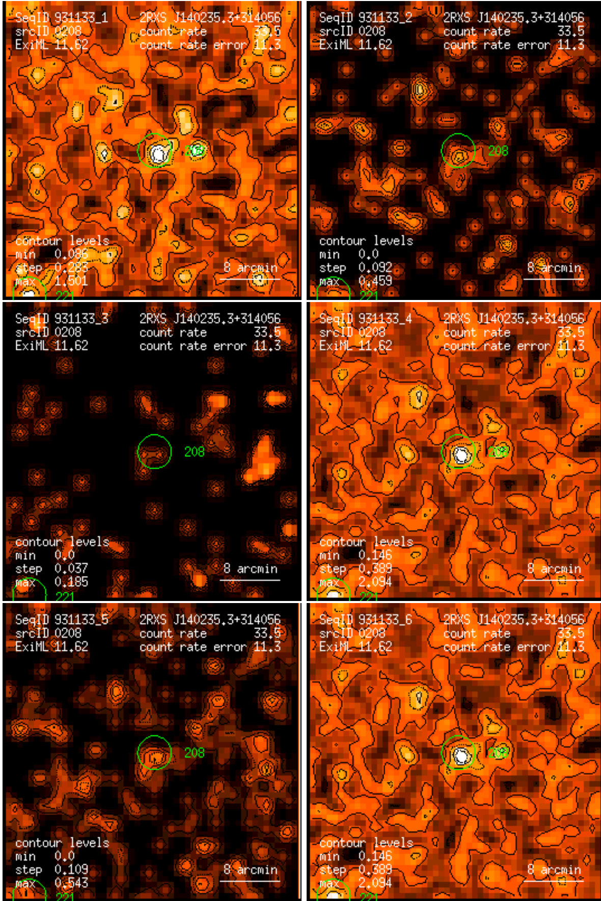
Figure 208: RASS 931133: detection 0208: band rate images, Gaussian filter: (1) PSPC channels 11 – 41, (2) 52 – 90, (3) 91 – 201, (4) 11 – 235, (5) 52 – 201, (6) 11 – 201. Broad band rates in counts/ks. Band rate contour levels in counts/ks/arcmin 2 .
