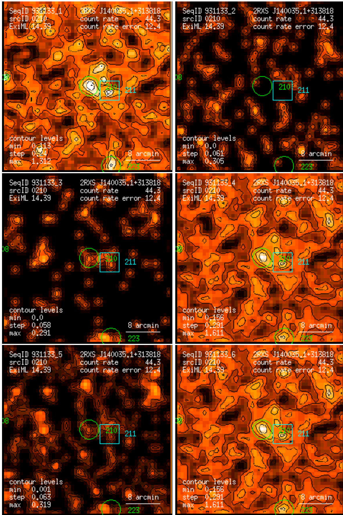
Figure 210: RASS 931133: detection 0210: band rate images, Gaussian filter: (1) PSPC channels 11 – 41, (2) 52 – 90, (3) 91 – 201, (4) 11 – 235, (5) 52 – 201, (6) 11 – 201. Broad band rates in counts/ks. Band rate contour levels in counts/ks/arcmin 2 .
