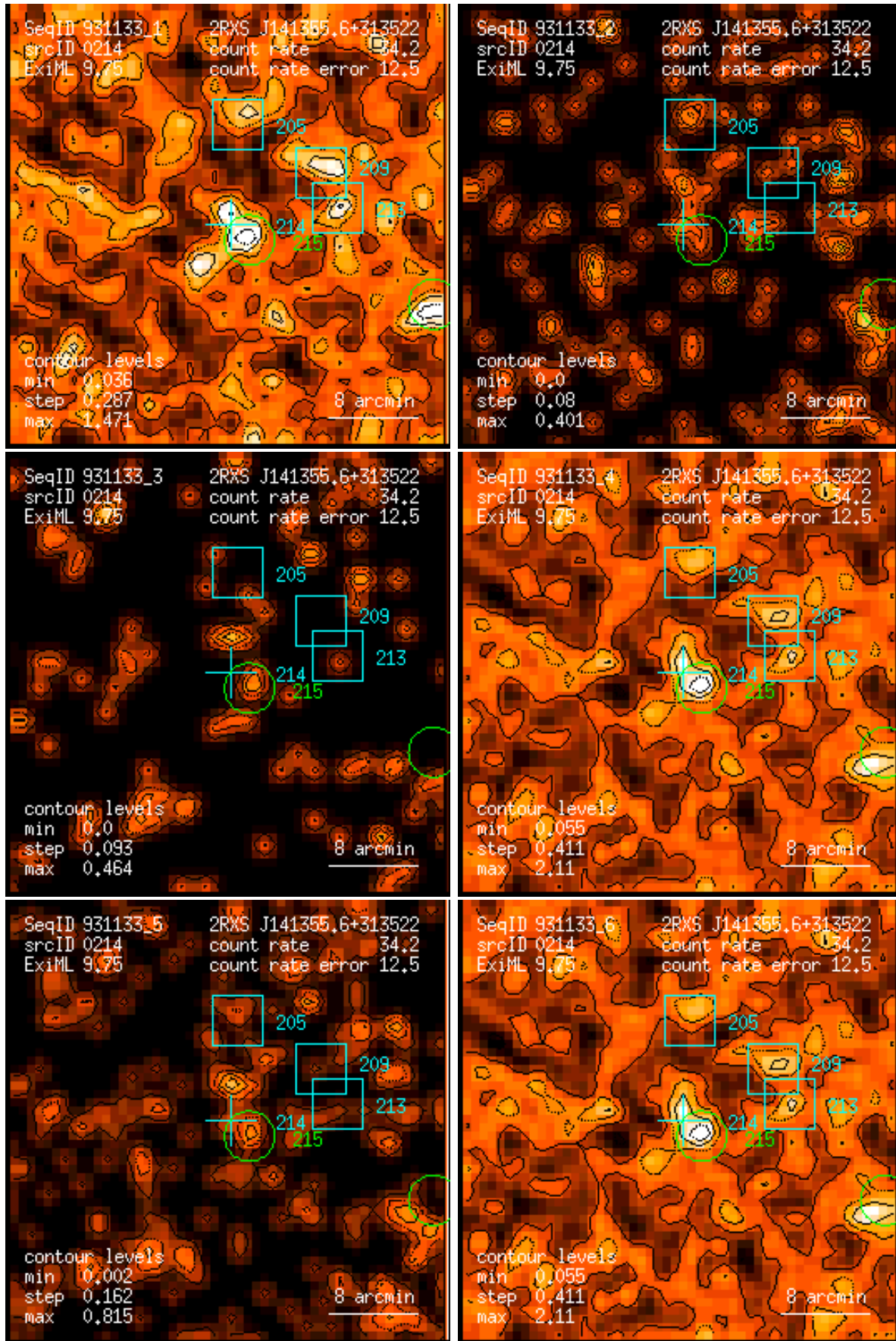
Figure 214: RASS 931133: detection 0214: band rate images, Gaussian filter: (1) PSPC channels 11 – 41, (2) 52 – 90, (3) 91 – 201, (4) 11 – 235, (5) 52 – 201, (6) 11 – 201. Broad band rates in counts/ks. Band rate contour levels in counts/ks/arcmin 2 .
