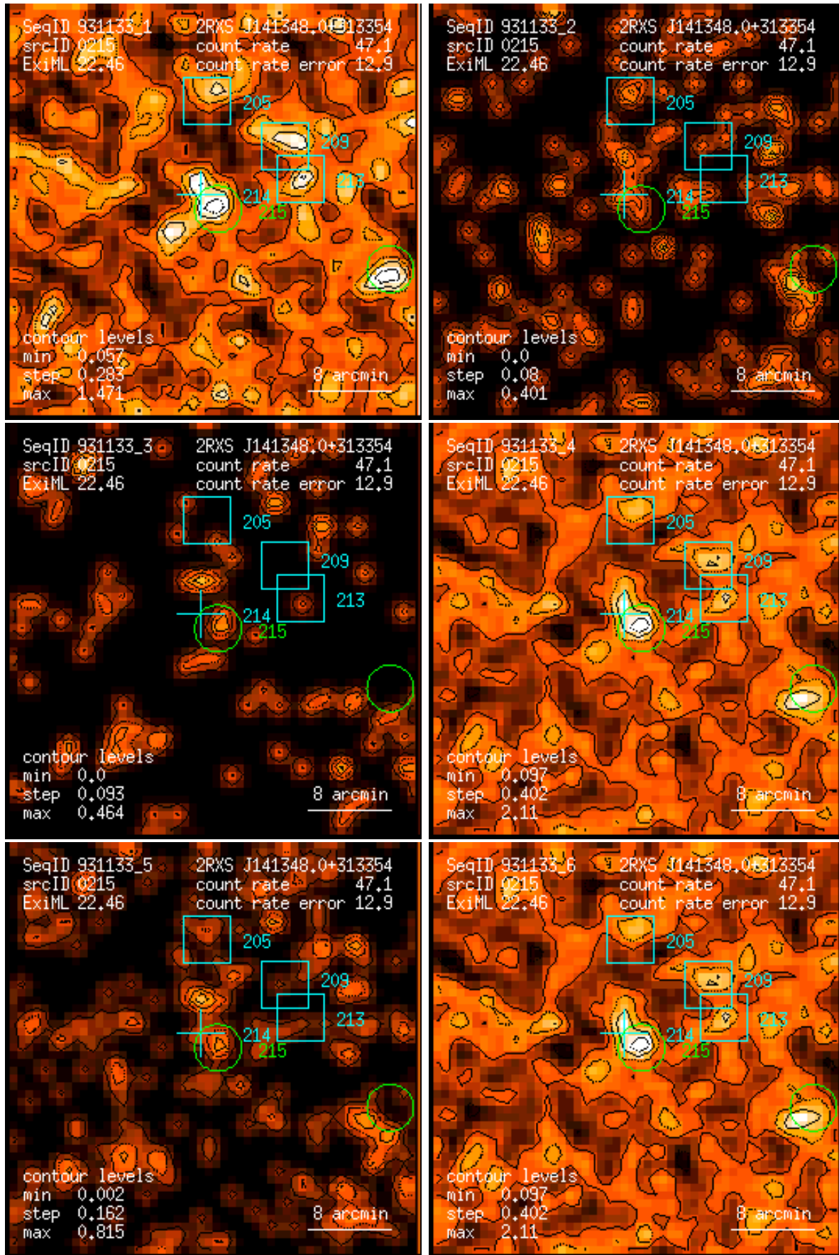
Figure 215: RASS 931133: detection 0215: band rate images, Gaussian filter: (1) PSPC channels 11 – 41, (2) 52 – 90, (3) 91 – 201, (4) 11 – 235, (5) 52 – 201, (6) 11 – 201. Broad band rates in counts/ks. Band rate contour levels in counts/ks/arcmin 2 .
