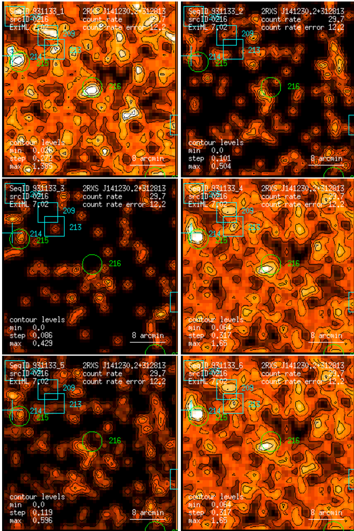
Figure 216: RASS 931133: detection 0216: band rate images, Gaussian filter: (1) PSPC channels 11 – 41, (2) 52 – 90, (3) 91 – 201, (4) 11 – 235, (5) 52 – 201, (6) 11 – 201. Broad band rates in counts/ks. Band rate contour levels in counts/ks/arcmin 2 .
