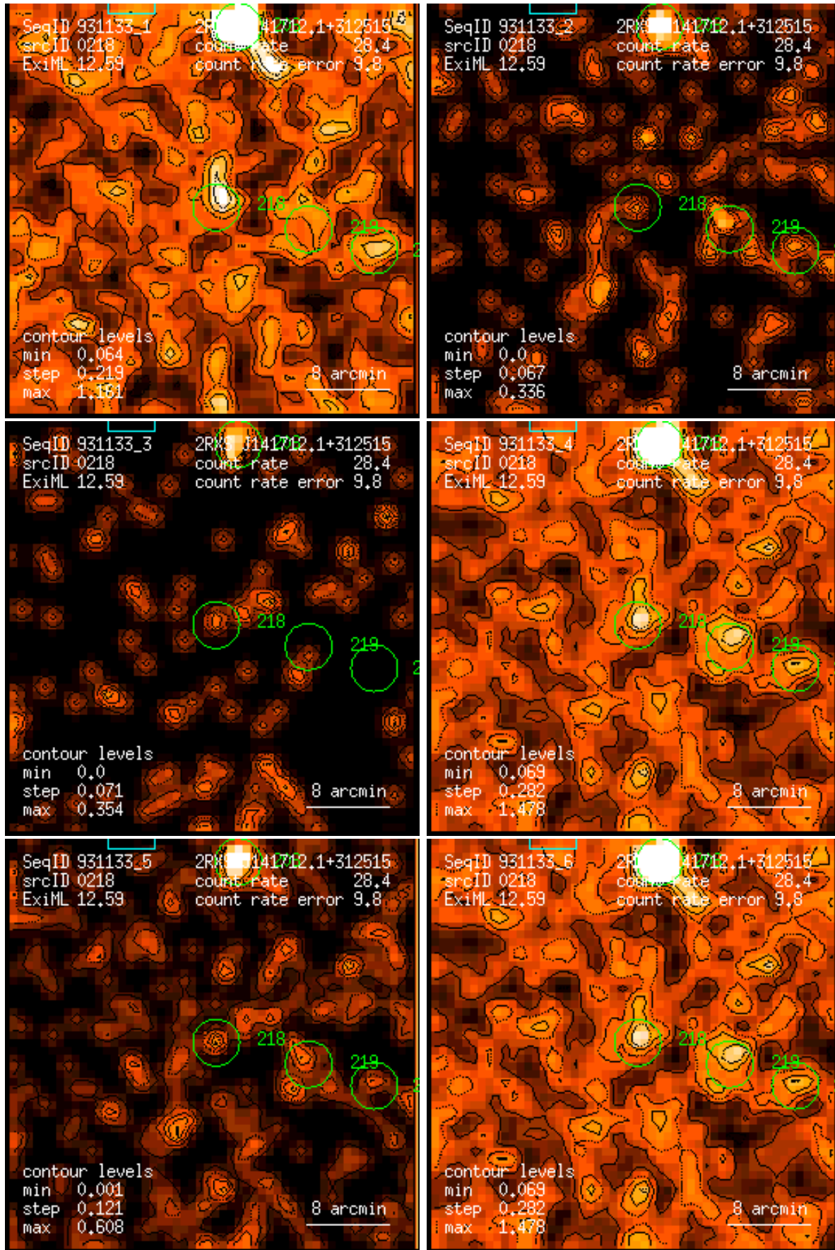
Figure 218: RASS 931133: detection 0218: band rate images, Gaussian filter: (1) PSPC channels 11 – 41, (2) 52 – 90, (3) 91 – 201, (4) 11 – 235, (5) 52 – 201, (6) 11 – 201. Broad band rates in counts/ks. Band rate contour levels in counts/ks/arcmin 2 .
