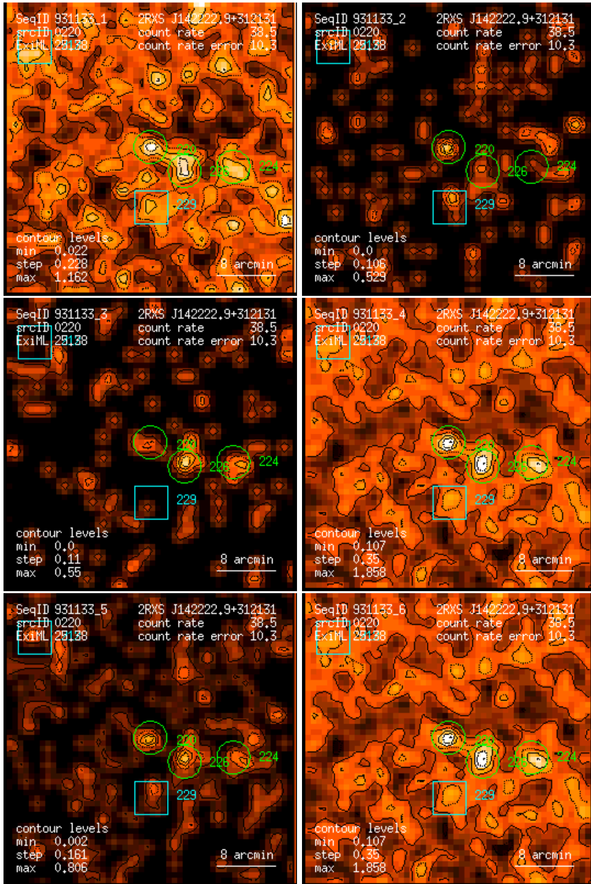
Figure 220: RASS 931133: detection 0220: band rate images, Gaussian filter: (1) PSPC channels 11 – 41, (2) 52 – 90, (3) 91 – 201, (4) 11 – 235, (5) 52 – 201, (6) 11 – 201. Broad band rates in counts/ks. Band rate contour levels in counts/ks/arcmin 2 .
