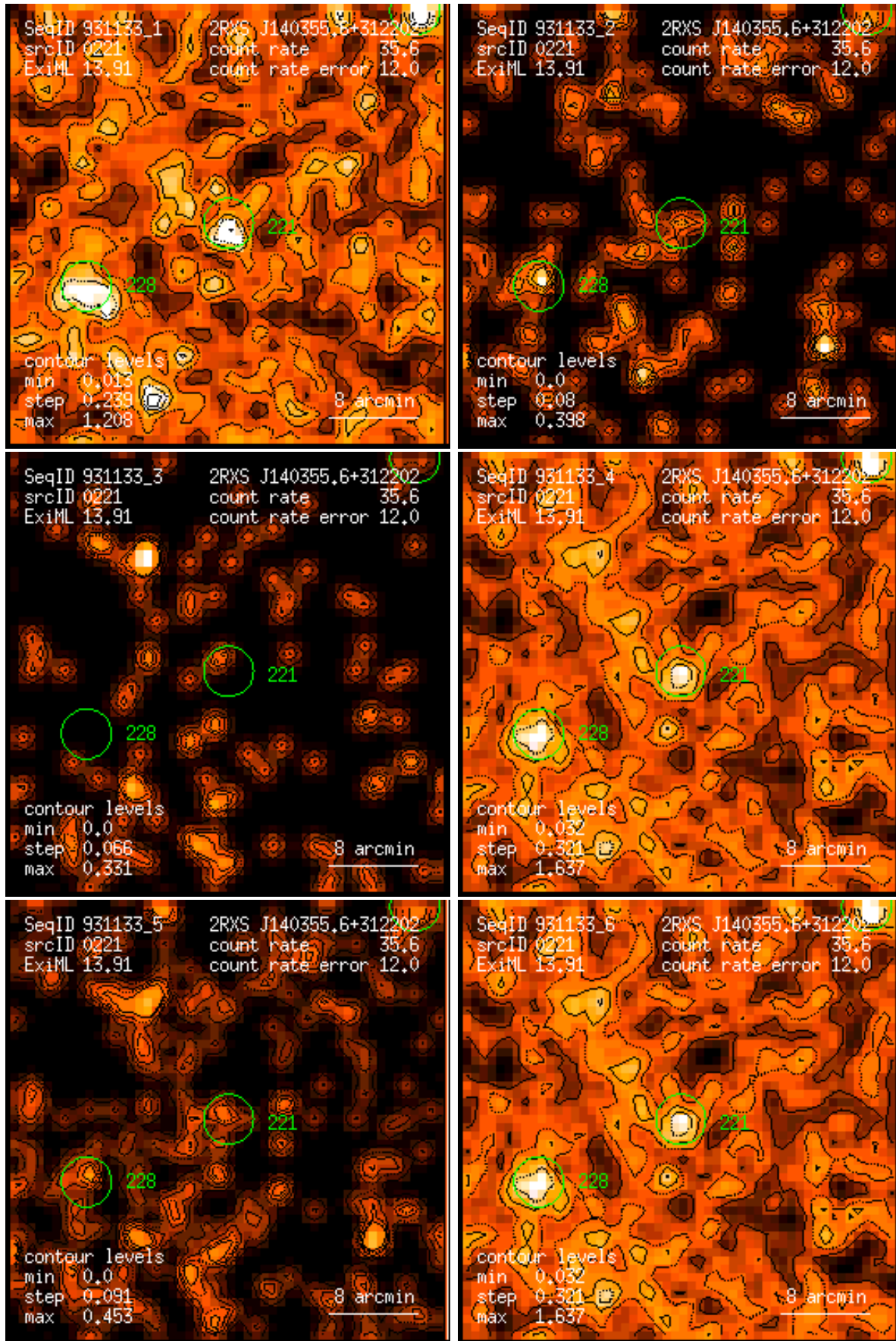
Figure 221: RASS 931133: detection 0221: band rate images, Gaussian filter: (1) PSPC channels 11 – 41, (2) 52 – 90, (3) 91 – 201, (4) 11 – 235, (5) 52 – 201, (6) 11 – 201. Broad band rates in counts/ks. Band rate contour levels in counts/ks/arcmin 2 .
