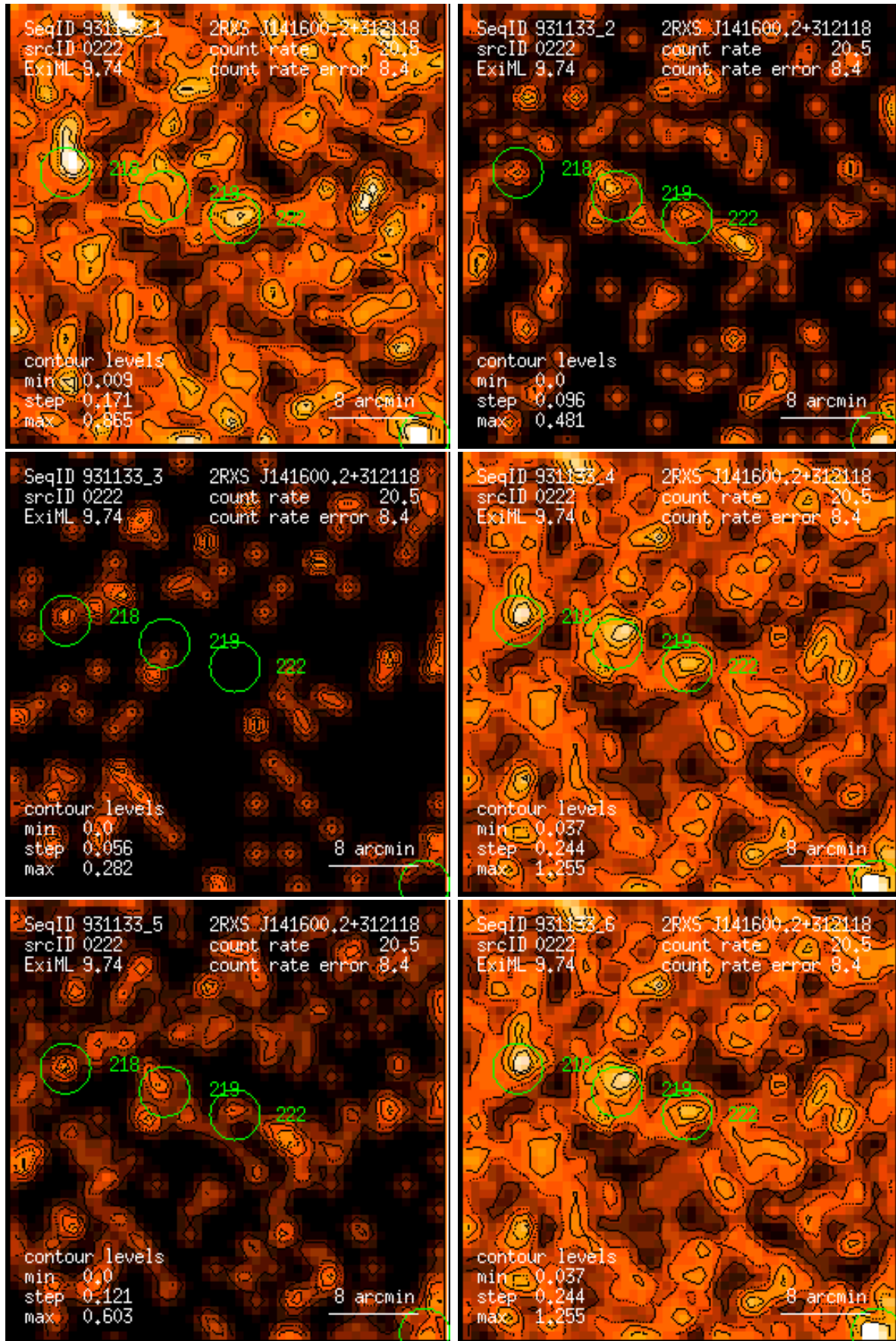
Figure 222: RASS 931133: detection 0222: band rate images, Gaussian filter: (1) PSPC channels 11 – 41, (2) 52 – 90, (3) 91 – 201, (4) 11 – 235, (5) 52 – 201, (6) 11 – 201. Broad band rates in counts/ks. Band rate contour levels in counts/ks/arcmin 2 .
