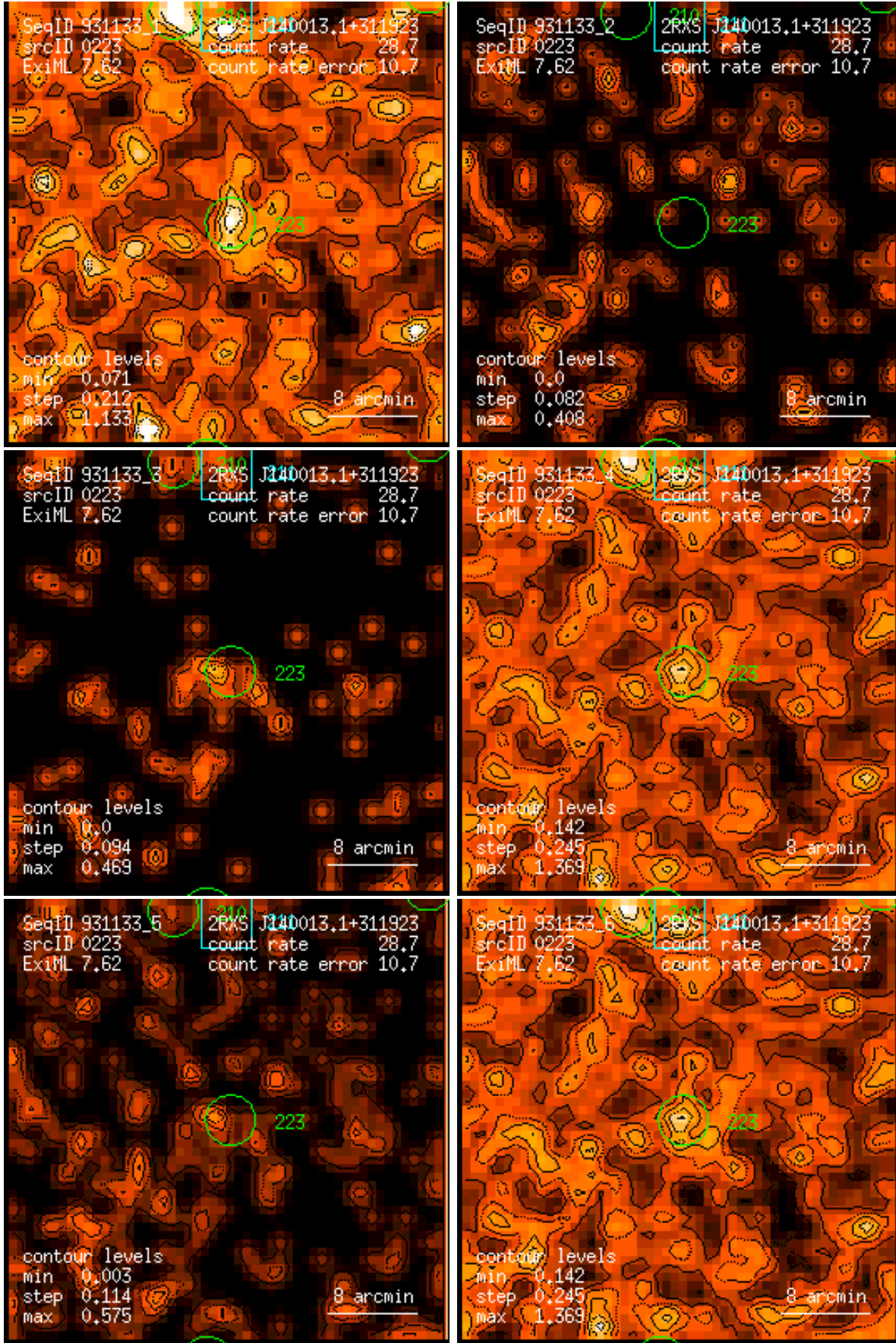
Figure 223: RASS 931133: detection 0223: band rate images, Gaussian filter: (1) PSPC channels 11 – 41, (2) 52 – 90, (3) 91 – 201, (4) 11 – 235, (5) 52 – 201, (6) 11 – 201. Broad band rates in counts/ks. Band rate contour levels in counts/ks/arcmin 2 .
