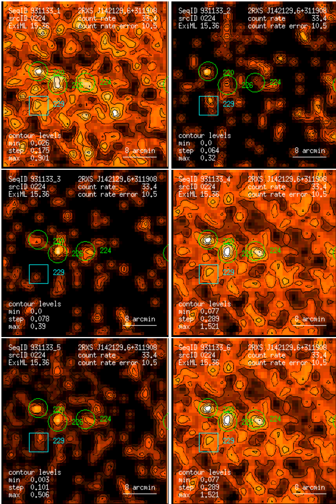
Figure 224: RASS 931133: detection 0224: band rate images, Gaussian filter: (1) PSPC channels 11 – 41, (2) 52 – 90, (3) 91 – 201, (4) 11 – 235, (5) 52 – 201, (6) 11 – 201. Broad band rates in counts/ks. Band rate contour levels in counts/ks/arcmin 2 .
