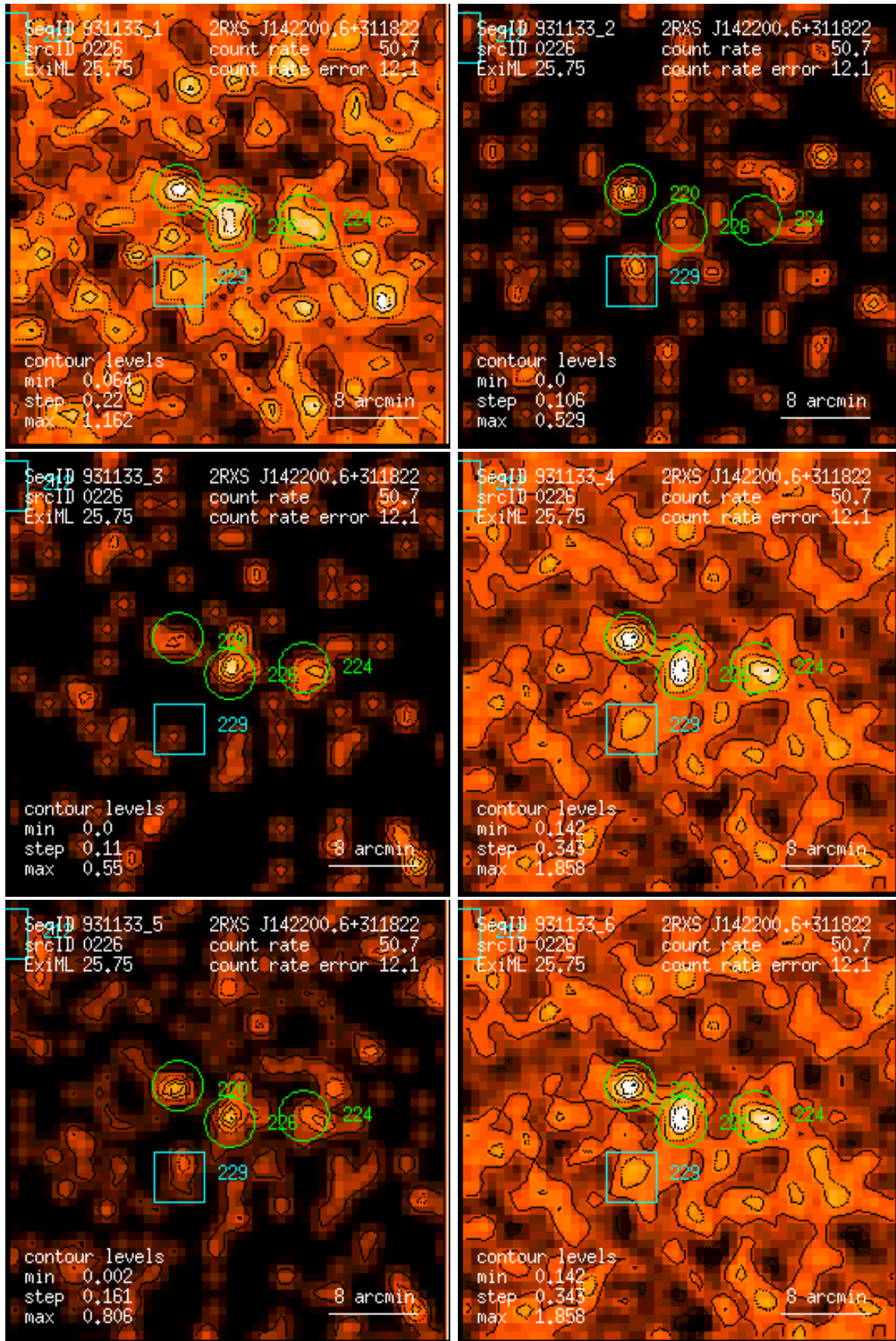
Figure 226: RASS 931133: detection 0226: band rate images, Gaussian filter: (1) PSPC channels 11 – 41, (2) 52 – 90, (3) 91 – 201, (4) 11 – 235, (5) 52 – 201, (6) 11 – 201. Broad band rates in counts/ks. Band rate contour levels in counts/ks/arcmin 2 .
