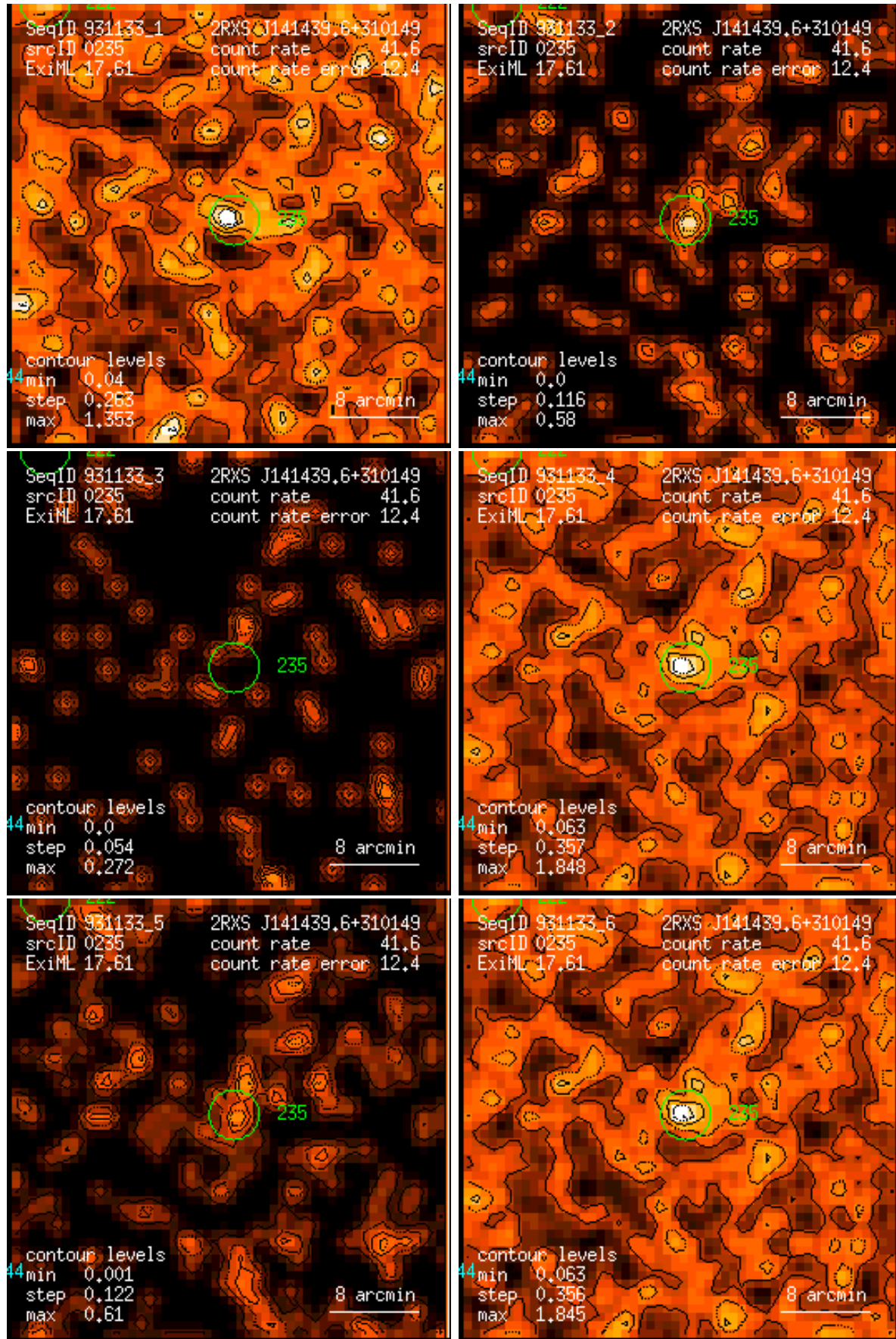
Figure 235: RASS 931133: detection 0235: band rate images, Gaussian filter: (1) PSPC channels 11 – 41, (2) 52 – 90, (3) 91 – 201, (4) 11 – 235, (5) 52 – 201, (6) 11 – 201. Broad band rates in counts/ks. Band rate contour levels in counts/ks/arcmin 2 .
