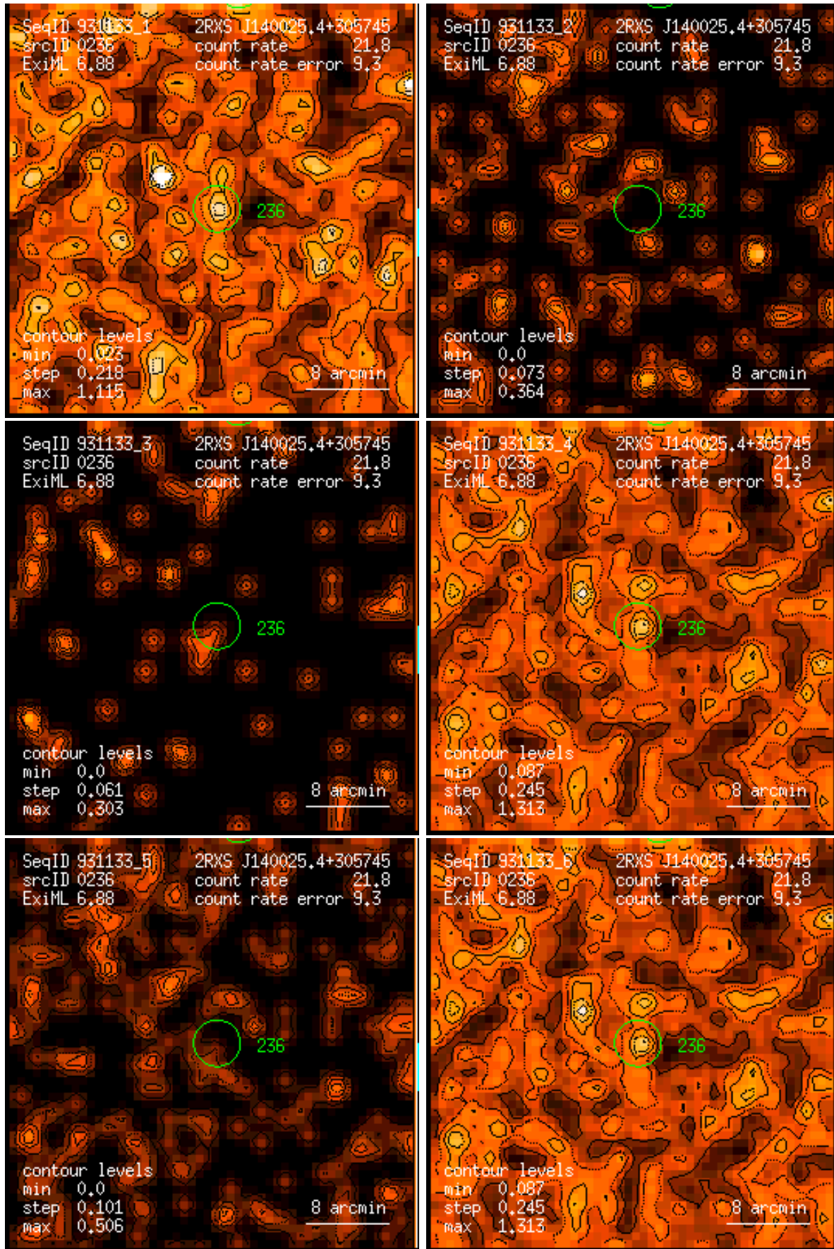
Figure 236: RASS 931133: detection 0236: band rate images, Gaussian filter: (1) PSPC channels 11 – 41, (2) 52 – 90, (3) 91 – 201, (4) 11 – 235, (5) 52 – 201, (6) 11 – 201. Broad band rates in counts/ks. Band rate contour levels in counts/ks/arcmin 2 .
