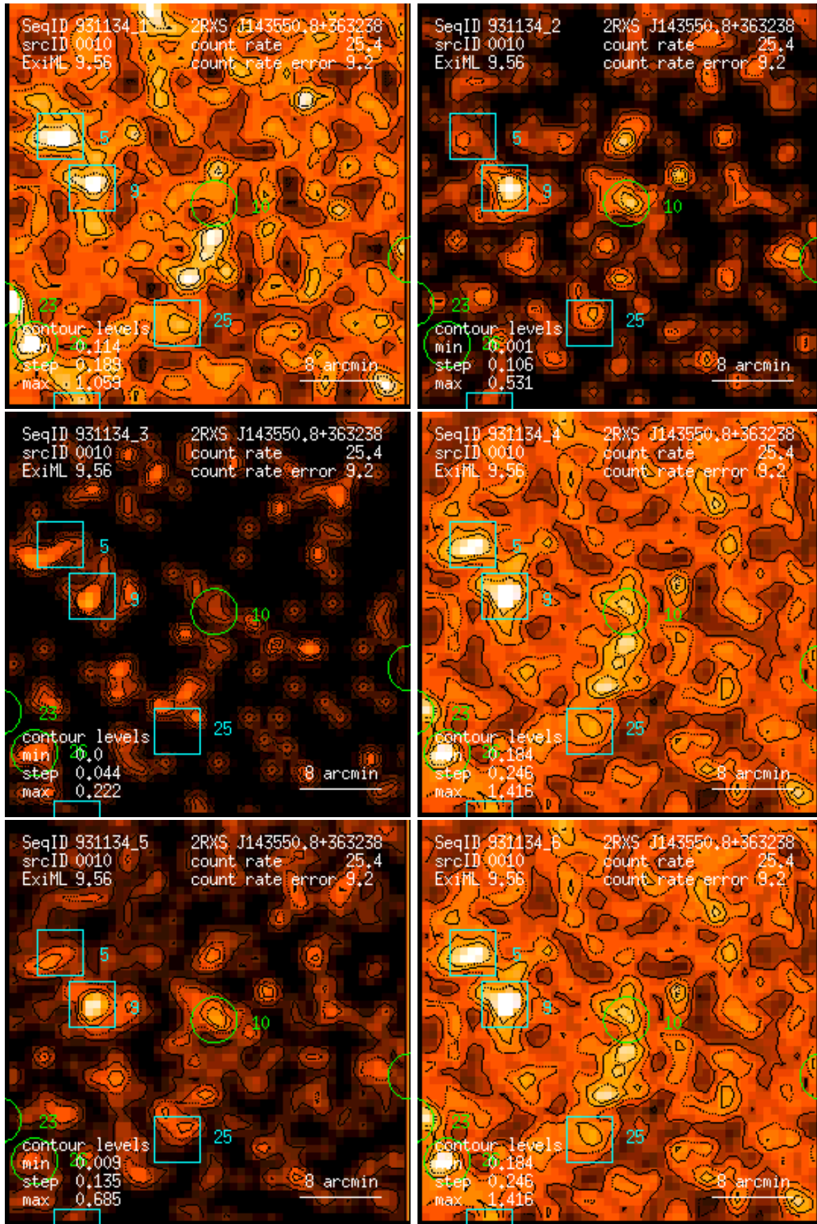
Figure 10: RASS 931134: detection 0010: band rate images, Gaussian filter: (1) PSPC channels 11 – 41, (2) 52 – 90, (3) 91 – 201, (4) 11 – 235, (5) 52 – 201, (6) 11 – 201. Broad band rates in counts/ks. Band rate contour levels in counts/ks/arcmin 2 .
