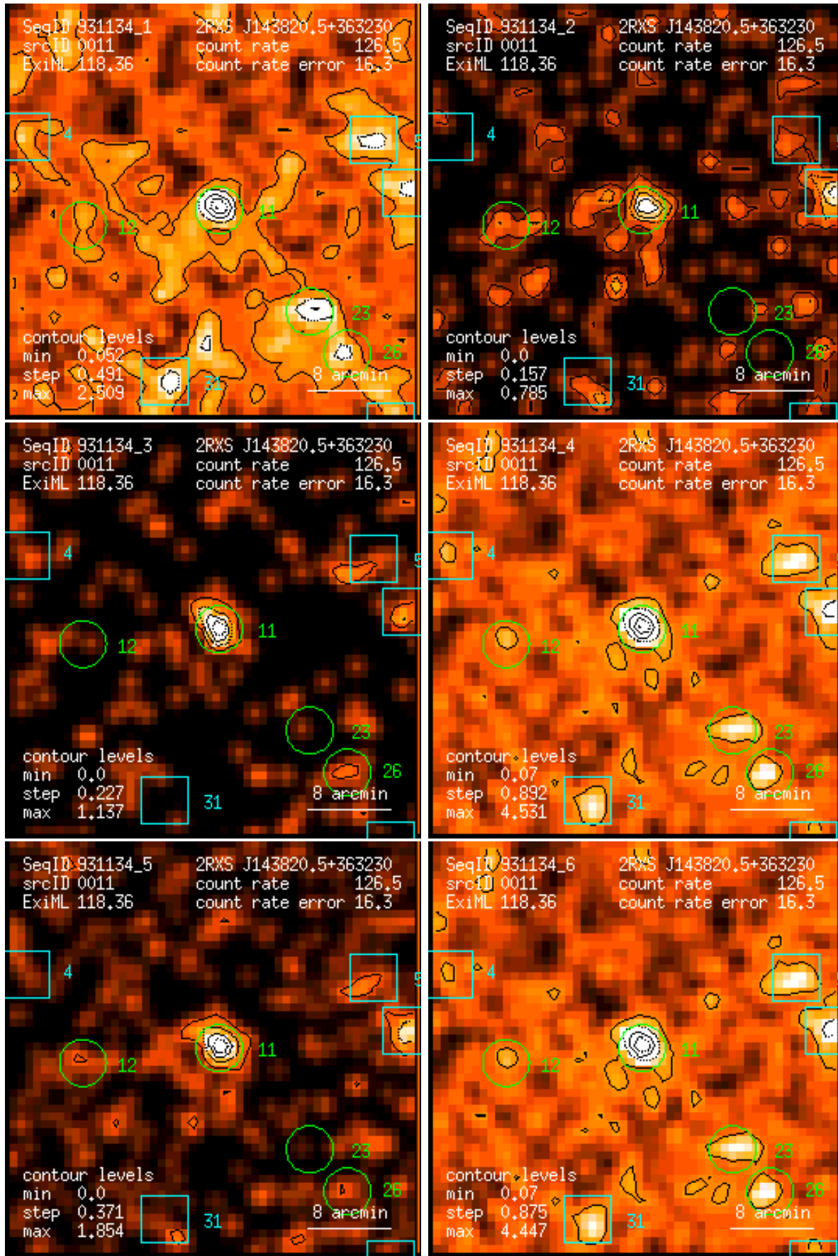
Figure 11: RASS 931134: detection 0011: band rate images, Gaussian filter: (1) PSPC channels 11 – 41, (2) 52 – 90, (3) 91 – 201, (4) 11 – 235, (5) 52 – 201, (6) 11 – 201. Broad band rates in counts/ks. Band rate contour levels in counts/ks/arcmin 2 .
