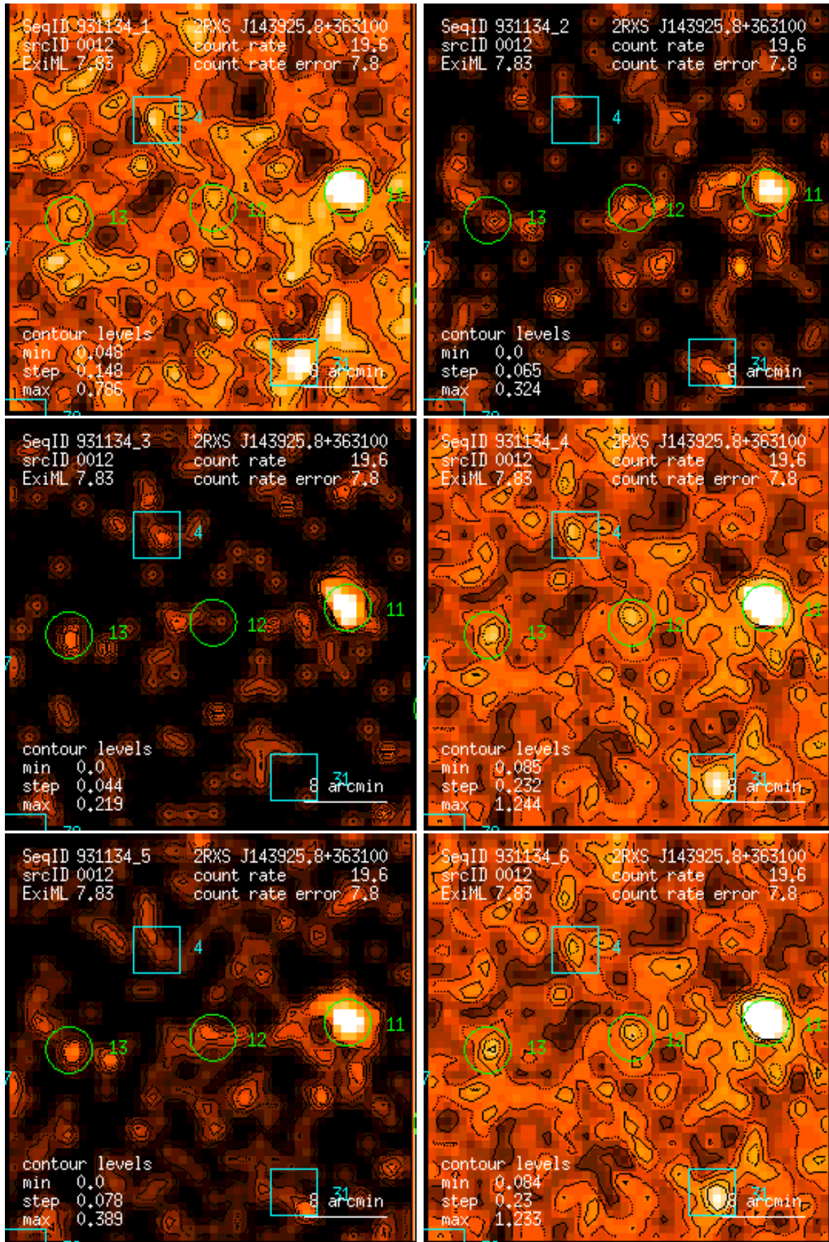
Figure 12: RASS 931134: detection 0012: band rate images, Gaussian filter: (1) PSPC channels 11 – 41, (2) 52 – 90, (3) 91 – 201, (4) 11 – 235, (5) 52 – 201, (6) 11 – 201. Broad band rates in counts/ks. Band rate contour levels in counts/ks/arcmin 2 .
