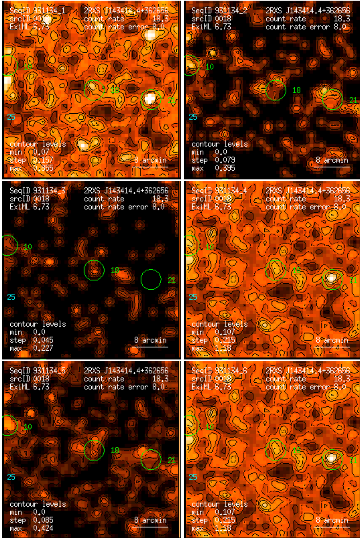
Figure 18: RASS 931134: detection 0018: band rate images, Gaussian filter: (1) PSPC channels 11 – 41, (2) 52 – 90, (3) 91 – 201, (4) 11 – 235, (5) 52 – 201, (6) 11 – 201. Broad band rates in counts/ks. Band rate contour levels in counts/ks/arcmin 2 .
