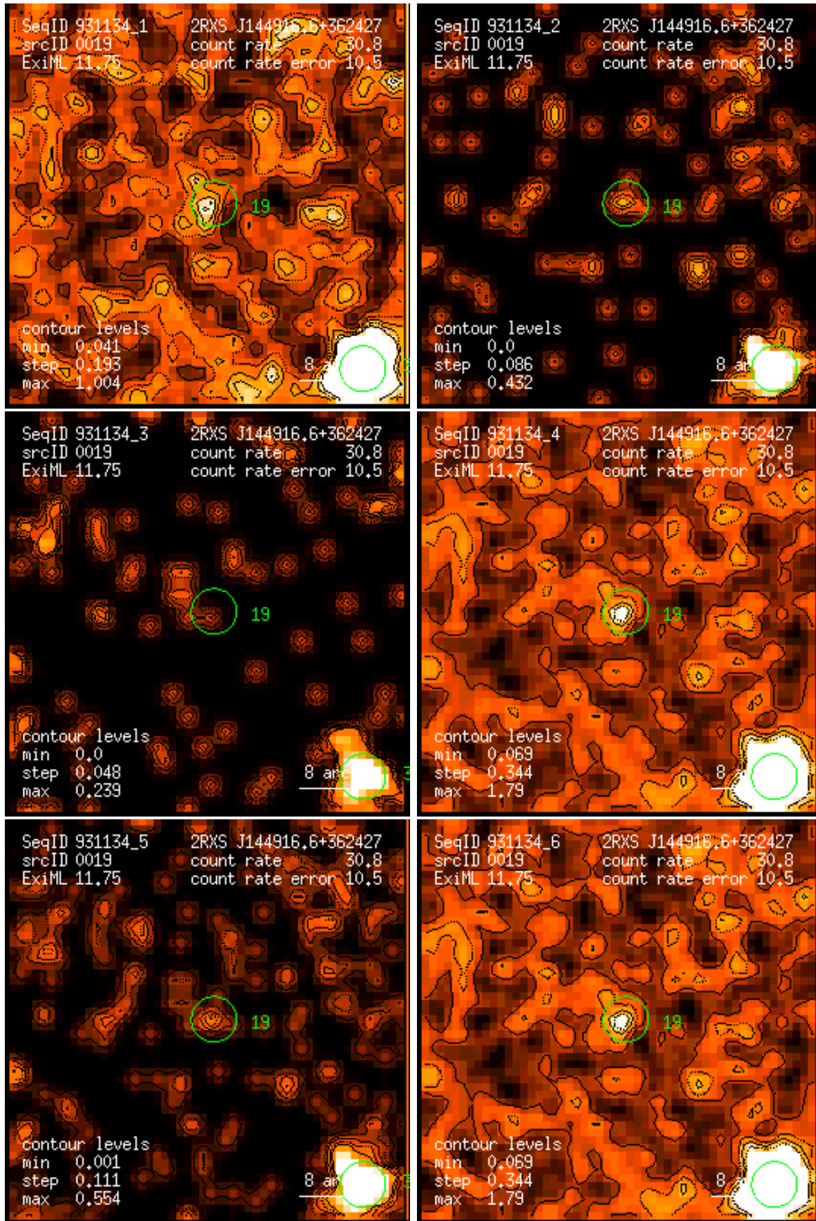
Figure 19: RASS 931134: detection 0019: band rate images, Gaussian filter: (1) PSPC channels 11 – 41, (2) 52 – 90, (3) 91 – 201, (4) 11 – 235, (5) 52 – 201, (6) 11 – 201. Broad band rates in counts/ks. Band rate contour levels in counts/ks/arcmin 2 .
