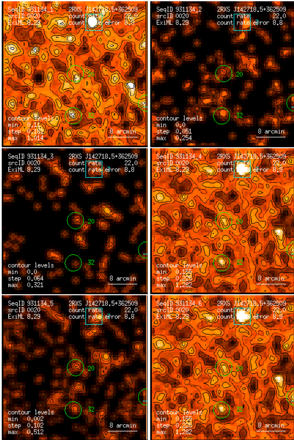
Figure 20: RASS 931134: detection 0020: band rate images, Gaussian filter: (1) PSPC channels 11 – 41, (2) 52 – 90, (3) 91 – 201, (4) 11 – 235, (5) 52 – 201, (6) 11 – 201. Broad band rates in counts/ks. Band rate contour levels in counts/ks/arcmin 2 .
