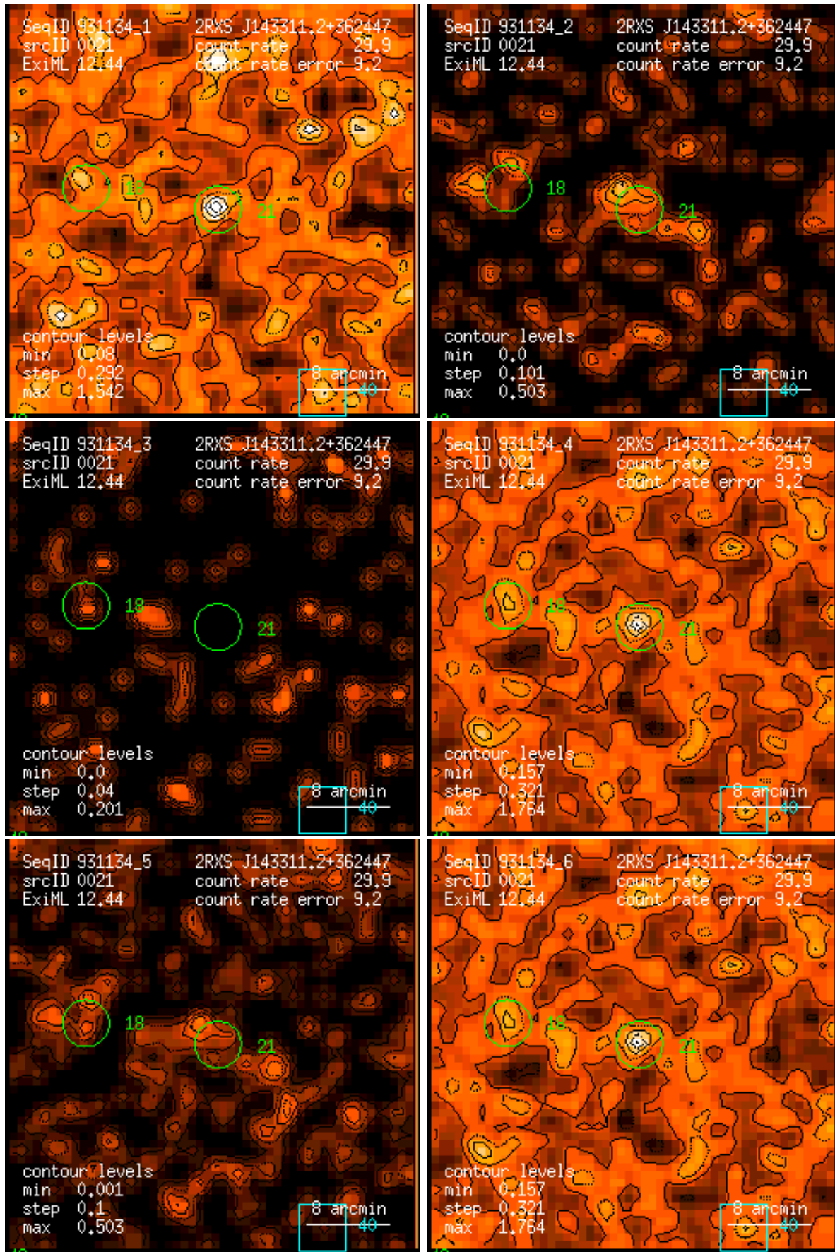
Figure 21: RASS 931134: detection 0021: band rate images, Gaussian filter: (1) PSPC channels 11 – 41, (2) 52 – 90, (3) 91 – 201, (4) 11 – 235, (5) 52 – 201, (6) 11 – 201. Broad band rates in counts/ks. Band rate contour levels in counts/ks/arcmin 2 .
